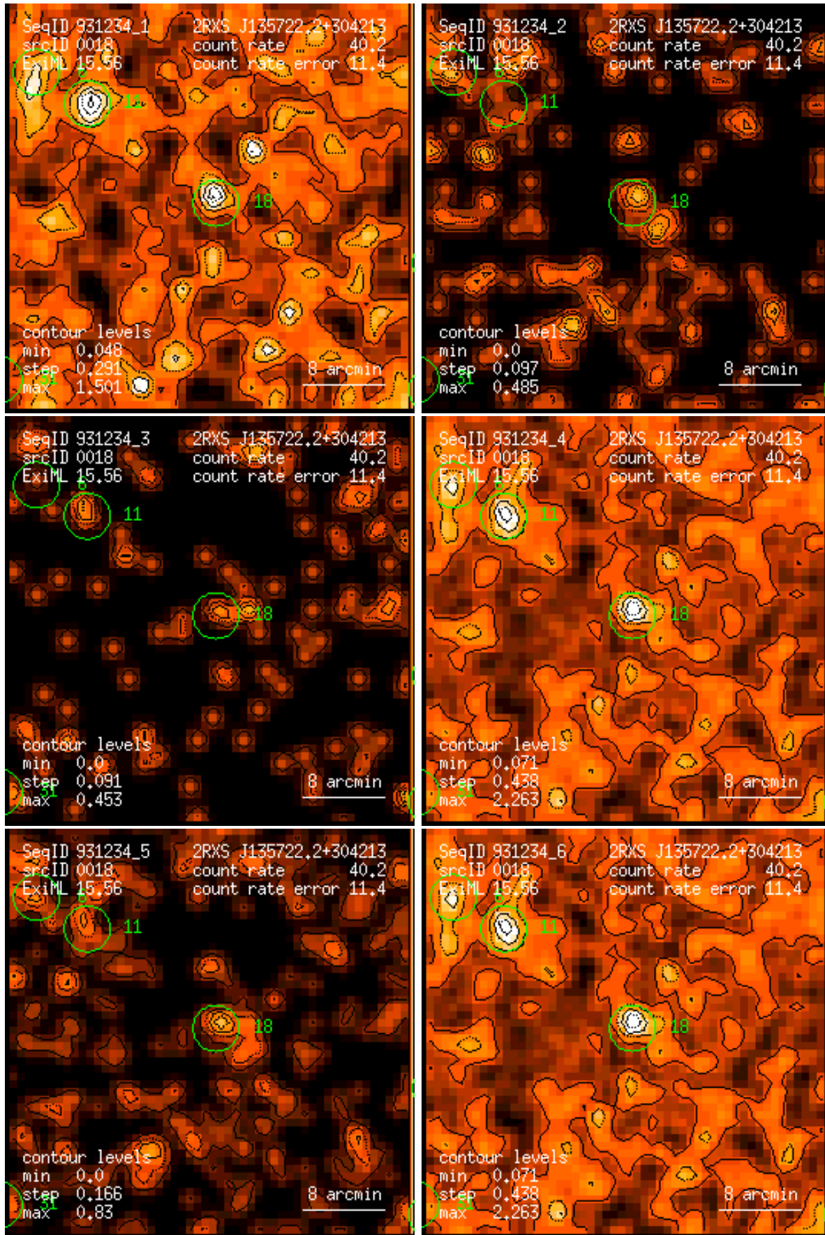
Figure 18: RASS 931234: detection 0018: band rate images, Gaussian filter: (1) PSPC channels 11 – 41, (2) 52 – 90, (3) 91 – 201, (4) 11 – 235, (5) 52 – 201, (6) 11 – 201. Broad band rates in counts/ks. Band rate contour levels in counts/ks/arcmin 2 .
