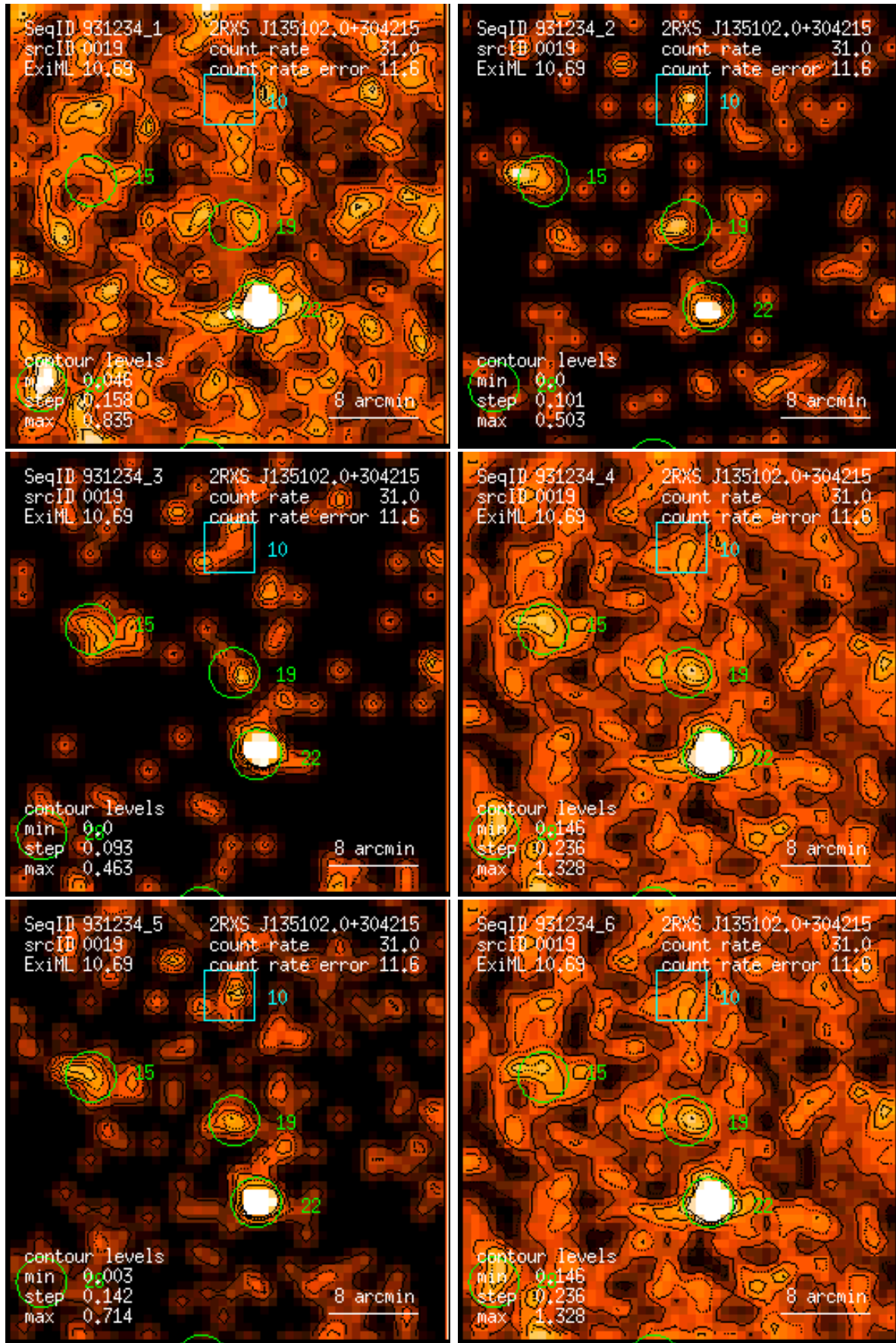
Figure 19: RASS 931234: detection 0019: band rate images, Gaussian filter: (1) PSPC channels 11 – 41, (2) 52 – 90, (3) 91 – 201, (4) 11 – 235, (5) 52 – 201, (6) 11 – 201. Broad band rates in counts/ks. Band rate contour levels in counts/ks/arcmin 2 .
