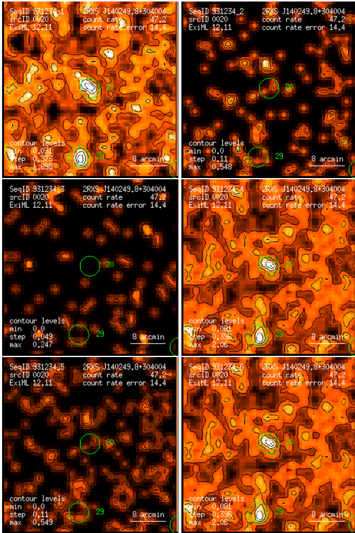
Figure 20: RASS 931234: detection 0020: band rate images, Gaussian filter: (1) PSPC channels 11 – 41, (2) 52 – 90, (3) 91 – 201, (4) 11 – 235, (5) 52 – 201, (6) 11 – 201. Broad band rates in counts/ks. Band rate contour levels in counts/ks/arcmin 2 .
