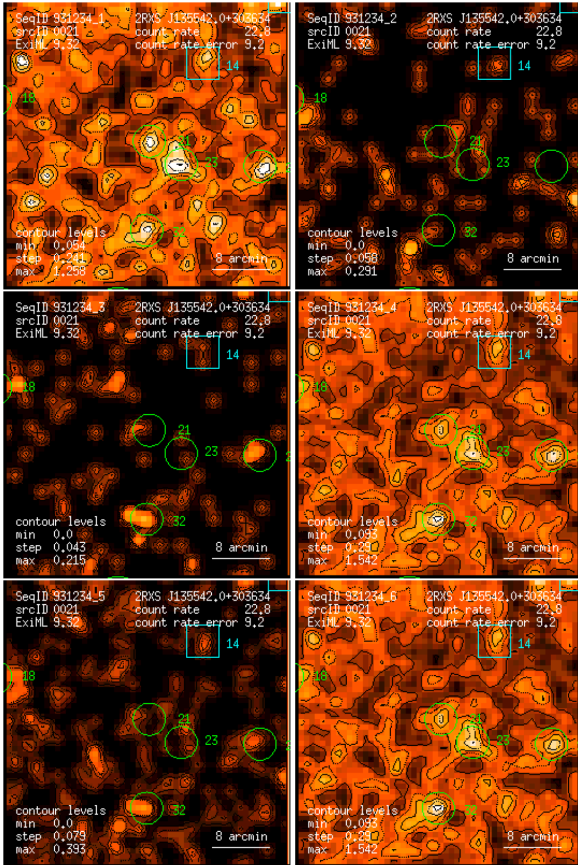
Figure 21: RASS 931234: detection 0021: band rate images, Gaussian filter: (1) PSPC channels 11 – 41, (2) 52 – 90, (3) 91 – 201, (4) 11 – 235, (5) 52 – 201, (6) 11 – 201. Broad band rates in counts/ks. Band rate contour levels in counts/ks/arcmin 2 .
