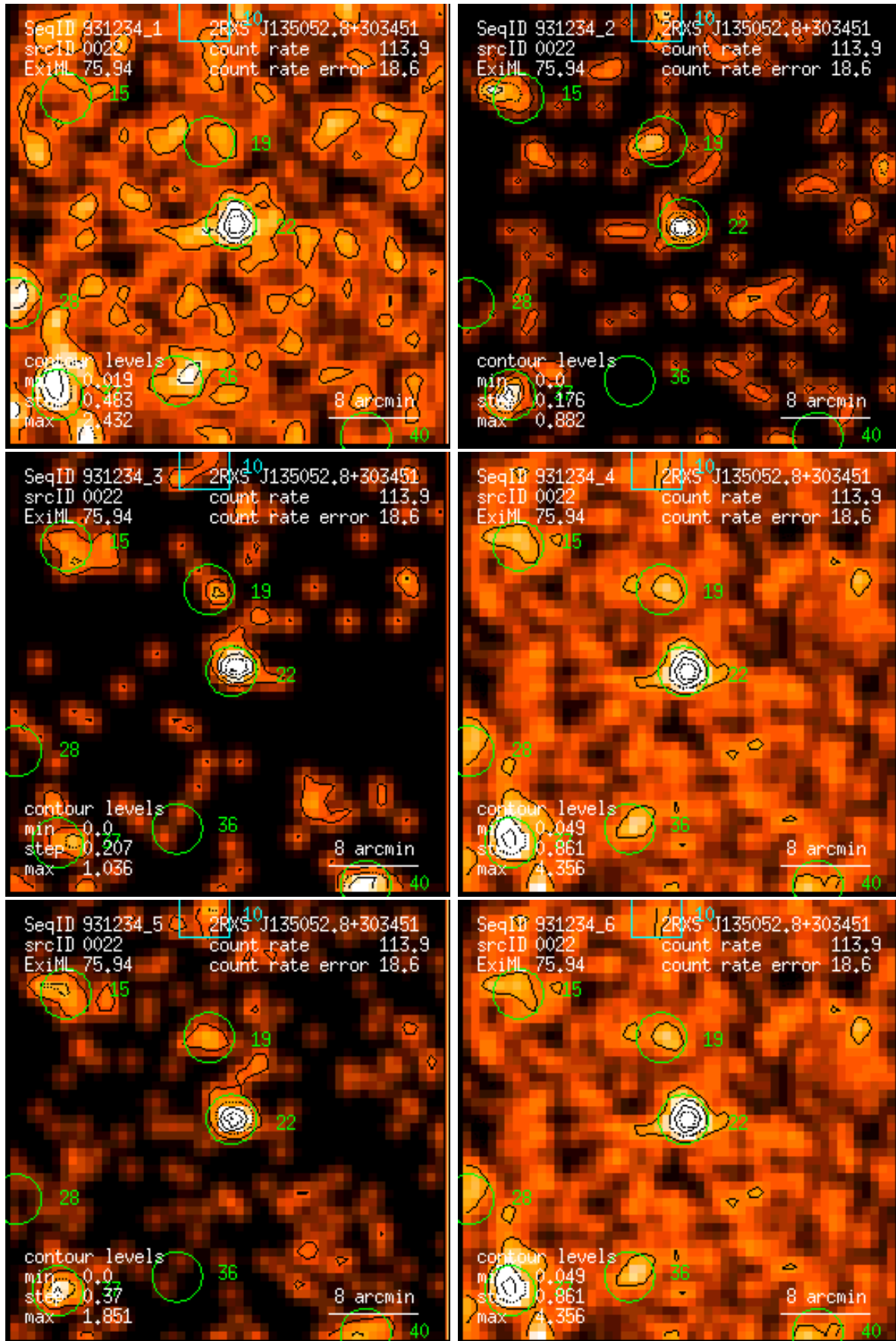
Figure 22: RASS 931234: detection 0022: band rate images, Gaussian filter: (1) PSPC channels 11 – 41, (2) 52 – 90, (3) 91 – 201, (4) 11 – 235, (5) 52 – 201, (6) 11 – 201. Broad band rates in counts/ks. Band rate contour levels in counts/ks/arcmin 2 .
