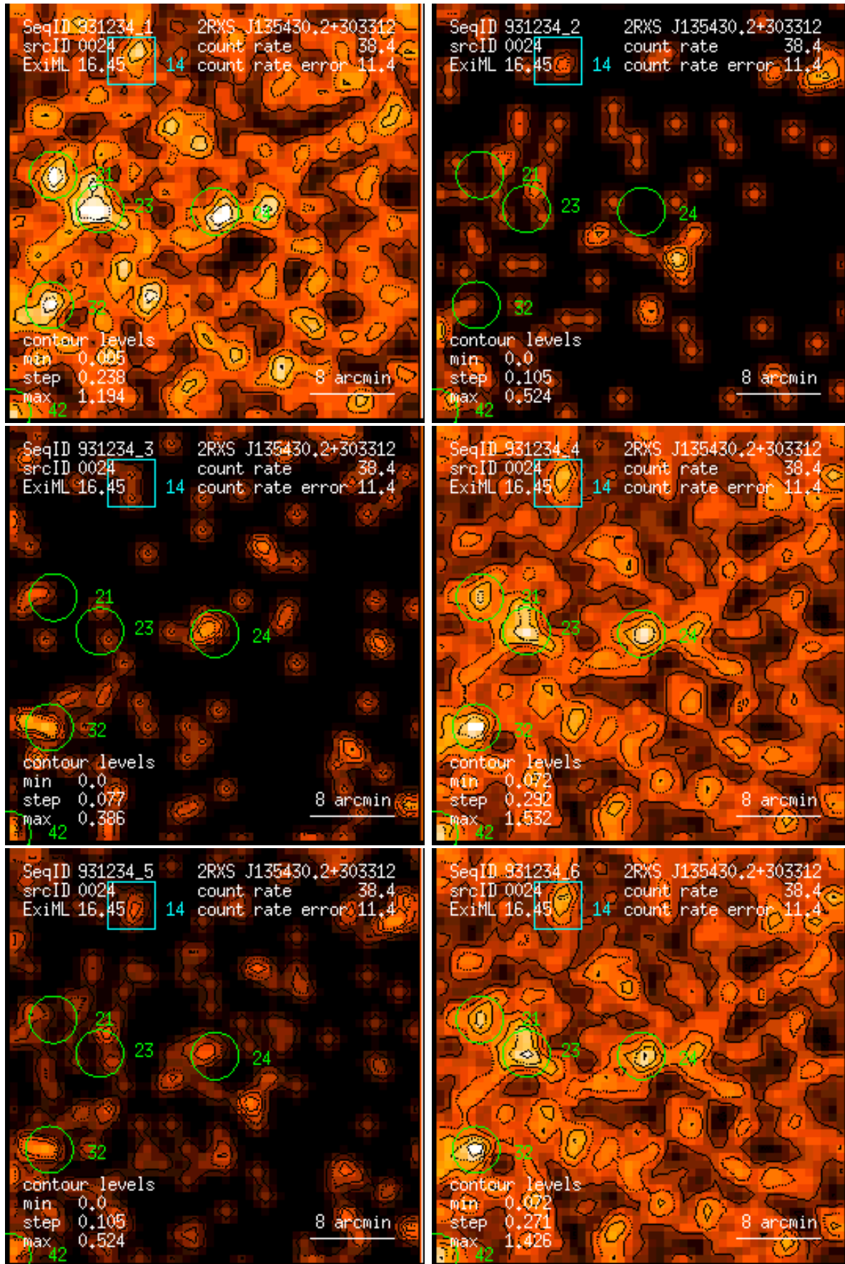
Figure 24: RASS 931234: detection 0024: band rate images, Gaussian filter: (1) PSPC channels 11 – 41, (2) 52 – 90, (3) 91 – 201, (4) 11 – 235, (5) 52 – 201, (6) 11 – 201. Broad band rates in counts/ks. Band rate contour levels in counts/ks/arcmin 2 .
