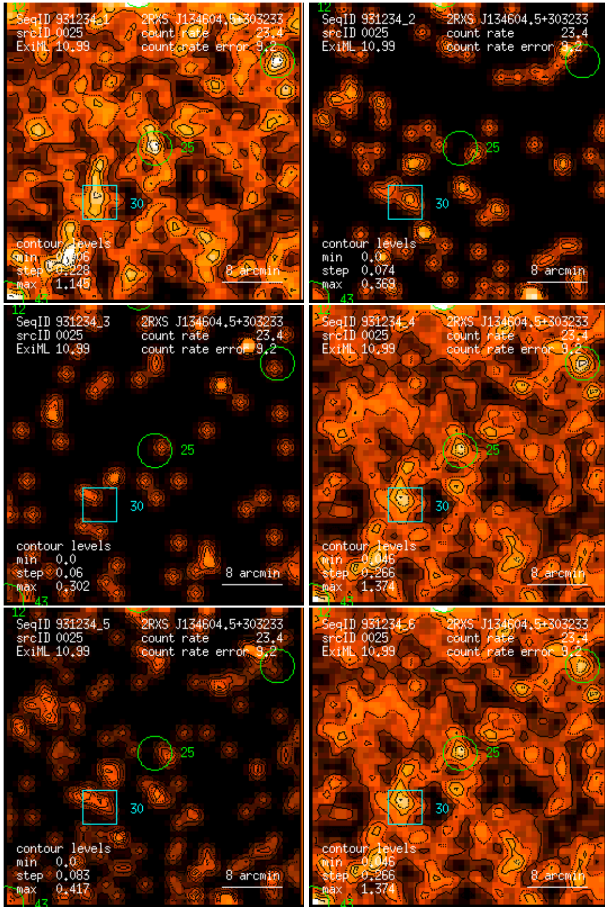
Figure 25: RASS 931234: detection 0025: band rate images, Gaussian filter: (1) PSPC channels 11 – 41, (2) 52 – 90, (3) 91 – 201, (4) 11 – 235, (5) 52 – 201, (6) 11 – 201. Broad band rates in counts/ks. Band rate contour levels in counts/ks/arcmin 2 .
