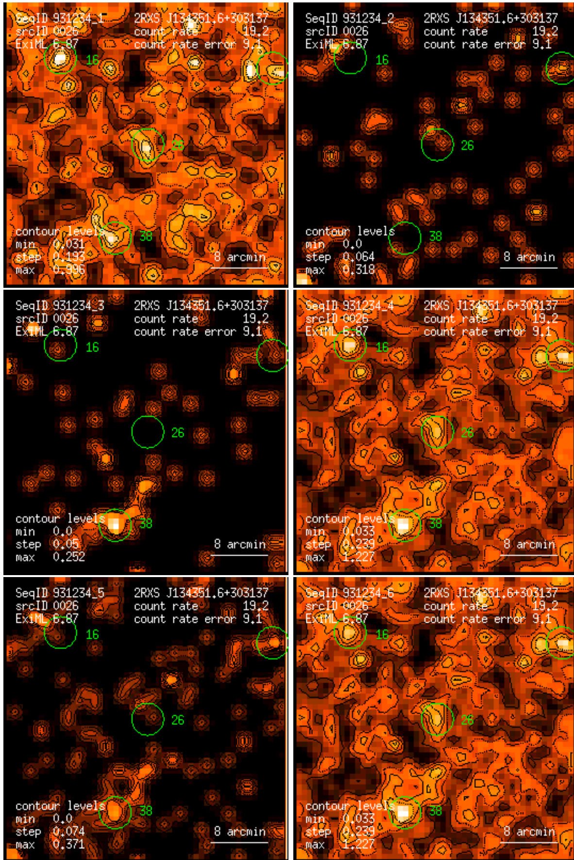
Figure 26: RASS 931234: detection 0026: band rate images, Gaussian filter: (1) PSPC channels 11 – 41, (2) 52 – 90, (3) 91 – 201, (4) 11 – 235, (5) 52 – 201, (6) 11 – 201. Broad band rates in counts/ks. Band rate contour levels in counts/ks/arcmin 2 .
