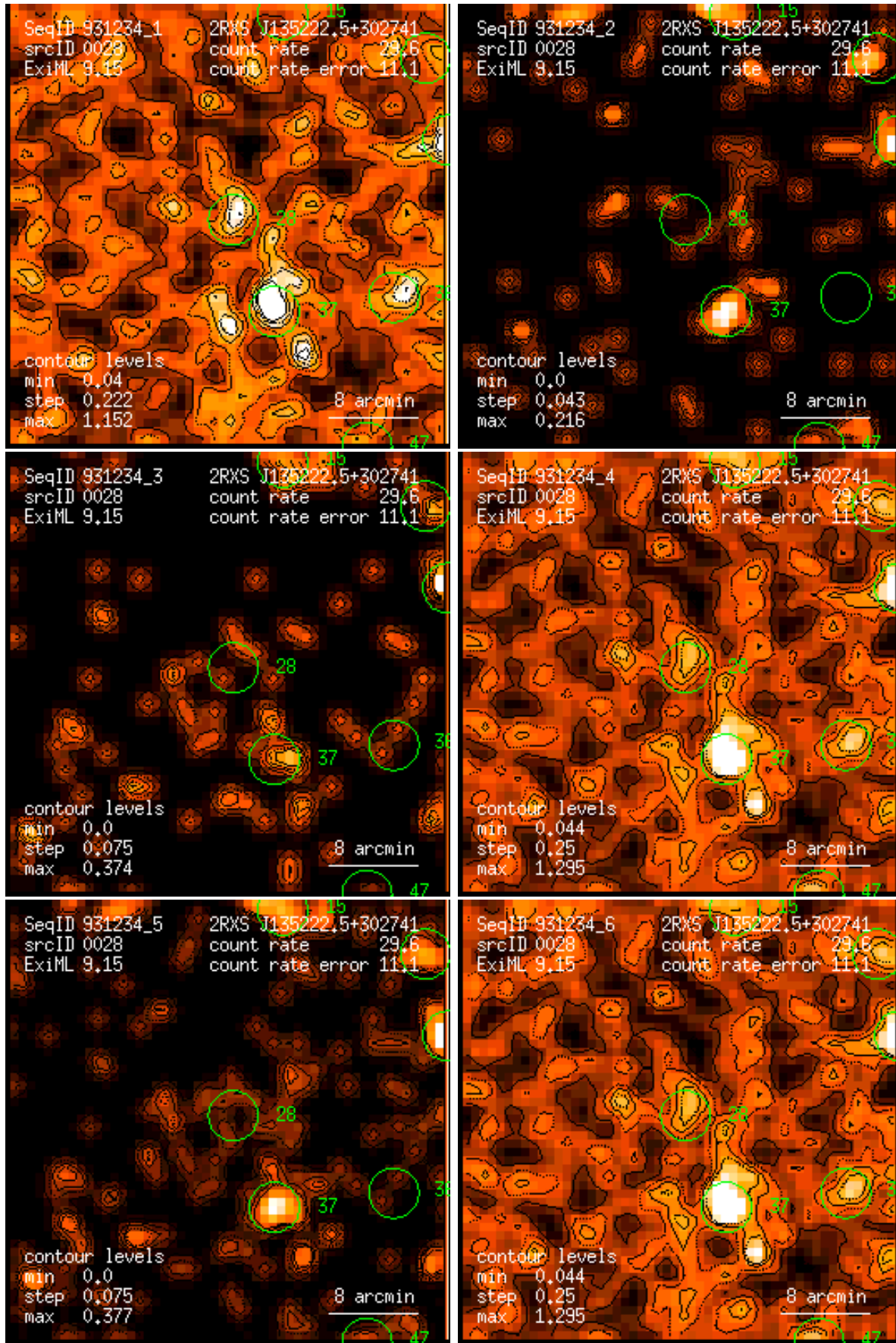
Figure 28: RASS 931234: detection 0028: band rate images, Gaussian filter: (1) PSPC channels 11 – 41, (2) 52 – 90, (3) 91 – 201, (4) 11 – 235, (5) 52 – 201, (6) 11 – 201. Broad band rates in counts/ks. Band rate contour levels in counts/ks/arcmin 2 .
