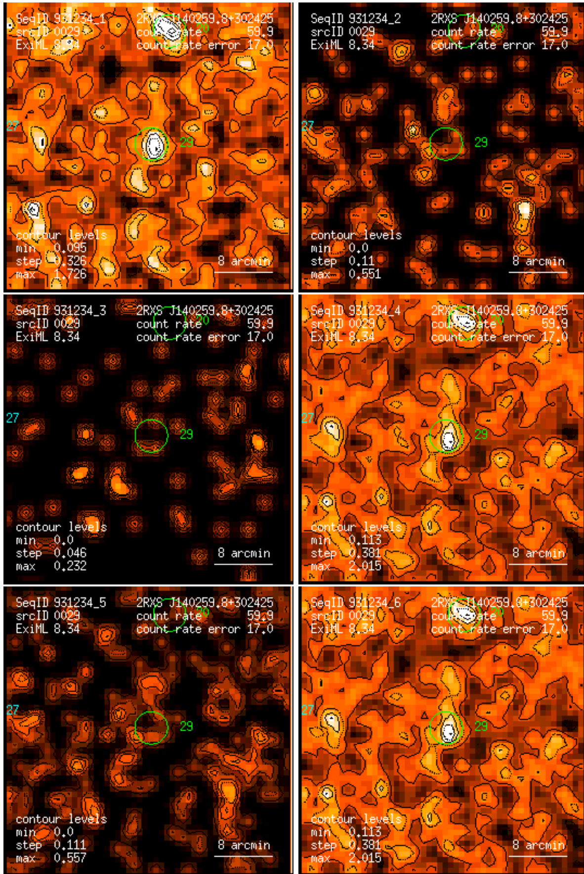
Figure 29: RASS 931234: detection 0029: band rate images, Gaussian filter: (1) PSPC channels 11 – 41, (2) 52 – 90, (3) 91 – 201, (4) 11 – 235, (5) 52 – 201, (6) 11 – 201. Broad band rates in counts/ks. Band rate contour levels in counts/ks/arcmin 2 .
