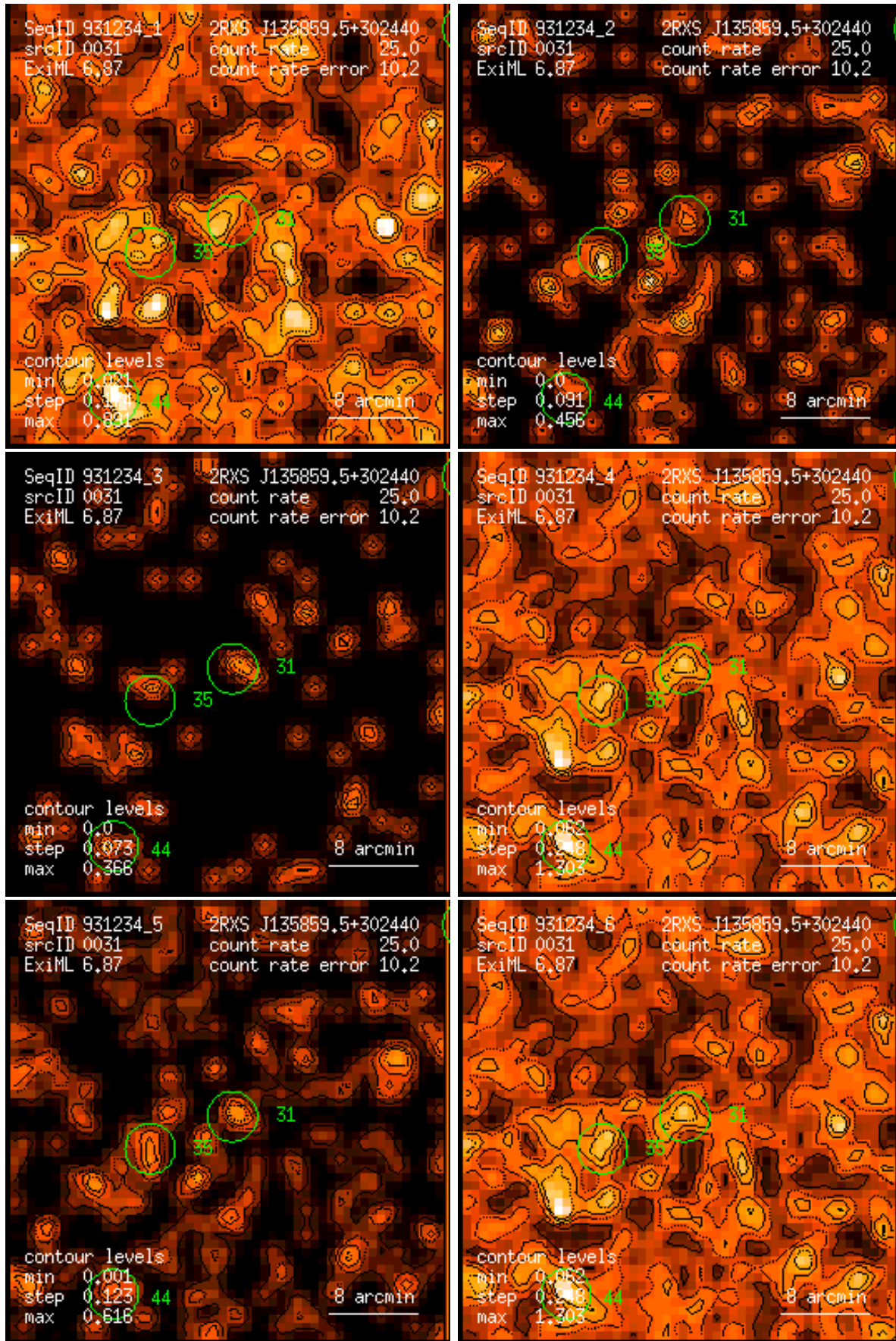
Figure 31: RASS 931234: detection 0031: band rate images, Gaussian filter: (1) PSPC channels 11 – 41, (2) 52 – 90, (3) 91 – 201, (4) 11 – 235, (5) 52 – 201, (6) 11 – 201. Broad band rates in counts/ks. Band rate contour levels in counts/ks/arcmin 2 .
