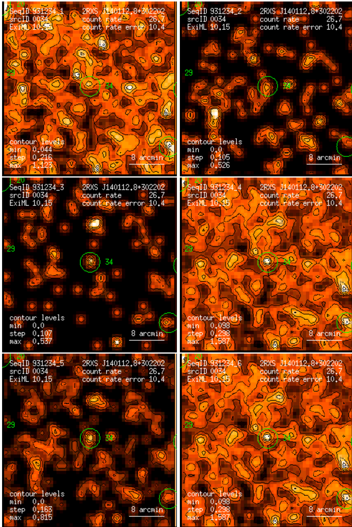
Figure 34: RASS 931234: detection 0034: band rate images, Gaussian filter: (1) PSPC channels 11 – 41, (2) 52 – 90, (3) 91 – 201, (4) 11 – 235, (5) 52 – 201, (6) 11 – 201. Broad band rates in counts/ks. Band rate contour levels in counts/ks/arcmin 2 .
