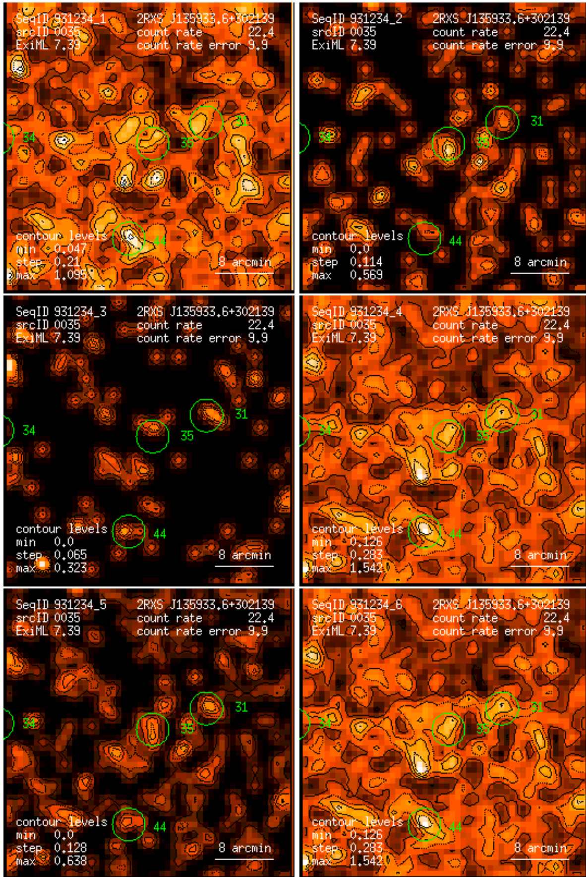
Figure 35: RASS 931234: detection 0035: band rate images, Gaussian filter: (1) PSPC channels 11 – 41, (2) 52 – 90, (3) 91 – 201, (4) 11 – 235, (5) 52 – 201, (6) 11 – 201. Broad band rates in counts/ks. Band rate contour levels in counts/ks/arcmin 2 .
