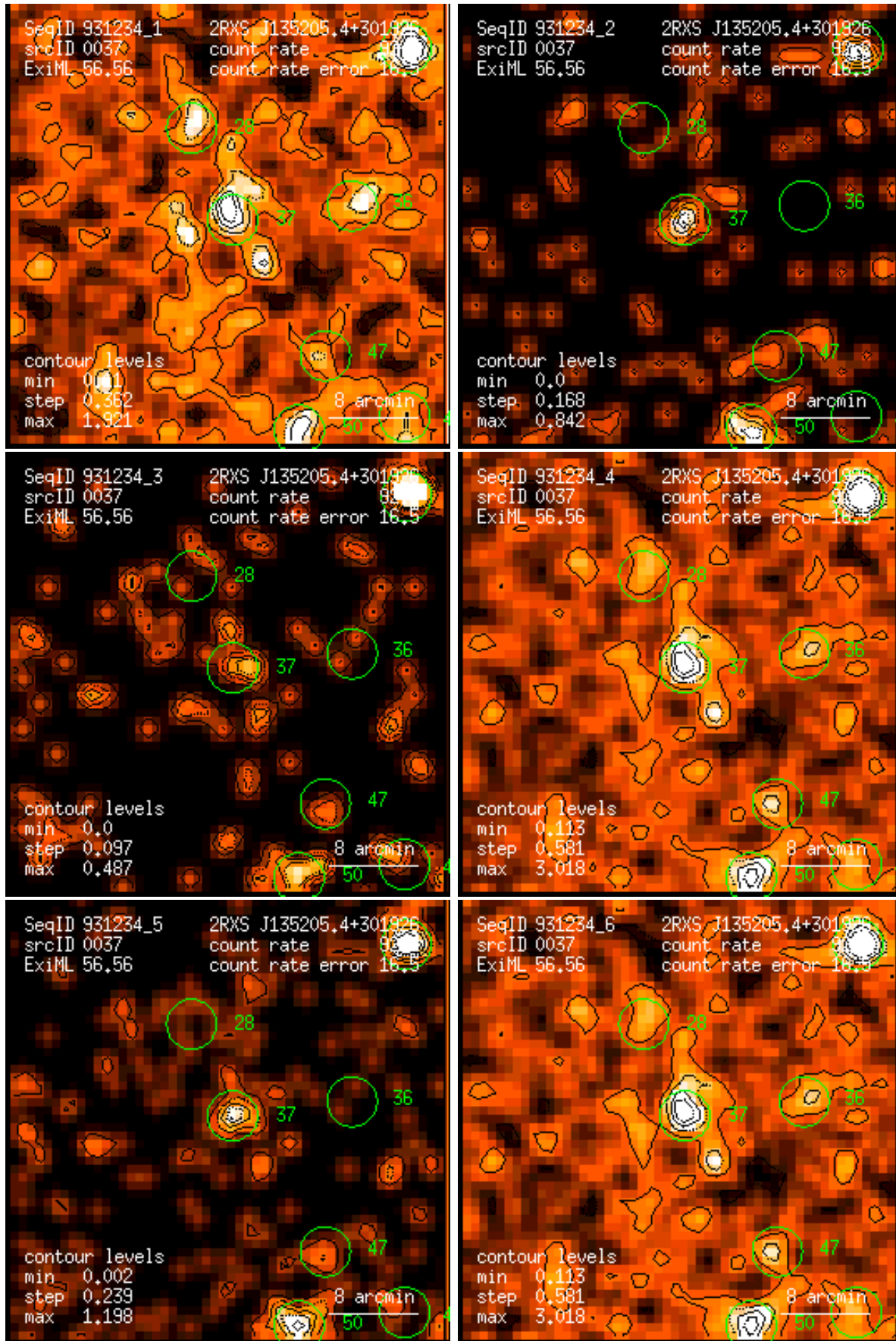
Figure 37: RASS 931234: detection 0037: band rate images, Gaussian filter: (1) PSPC channels 11 – 41, (2) 52 – 90, (3) 91 – 201, (4) 11 – 235, (5) 52 – 201, (6) 11 – 201. Broad band rates in counts/ks. Band rate contour levels in counts/ks/arcmin 2 .
