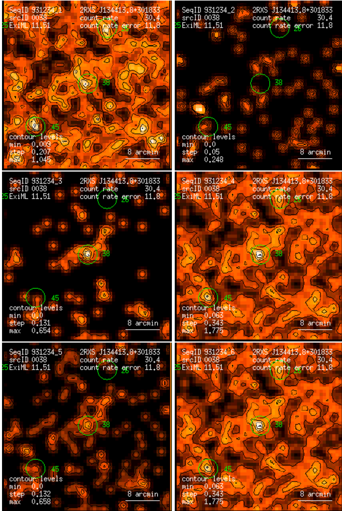
Figure 38: RASS 931234: detection 0038: band rate images, Gaussian filter: (1) PSPC channels 11 – 41, (2) 52 – 90, (3) 91 – 201, (4) 11 – 235, (5) 52 – 201, (6) 11 – 201. Broad band rates in counts/ks. Band rate contour levels in counts/ks/arcmin 2 .
