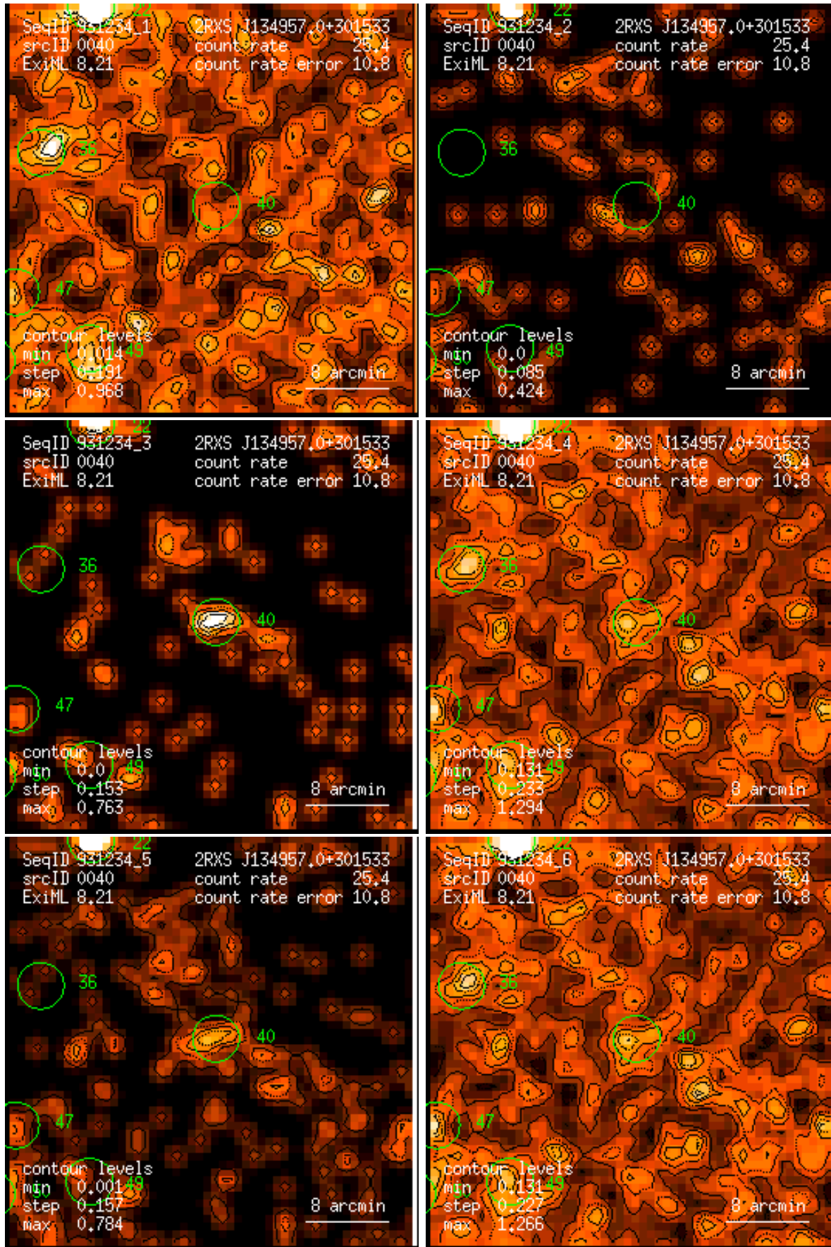
Figure 40: RASS 931234: detection 0040: band rate images, Gaussian filter: (1) PSPC channels 11 – 41, (2) 52 – 90, (3) 91 – 201, (4) 11 – 235, (5) 52 – 201, (6) 11 – 201. Broad band rates in counts/ks. Band rate contour levels in counts/ks/arcmin 2 .
