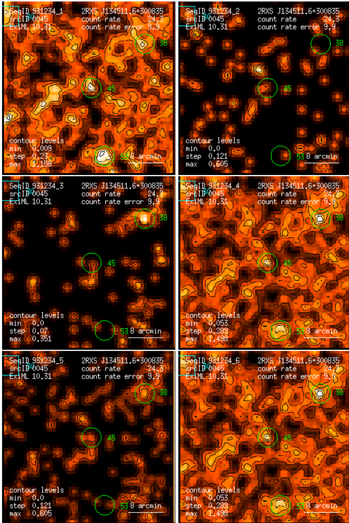
Figure 45: RASS 931234: detection 0045: band rate images, Gaussian filter: (1) PSPC channels 11 – 41, (2) 52 – 90, (3) 91 – 201, (4) 11 – 235, (5) 52 – 201, (6) 11 – 201. Broad band rates in counts/ks. Band rate contour levels in counts/ks/arcmin 2 .
