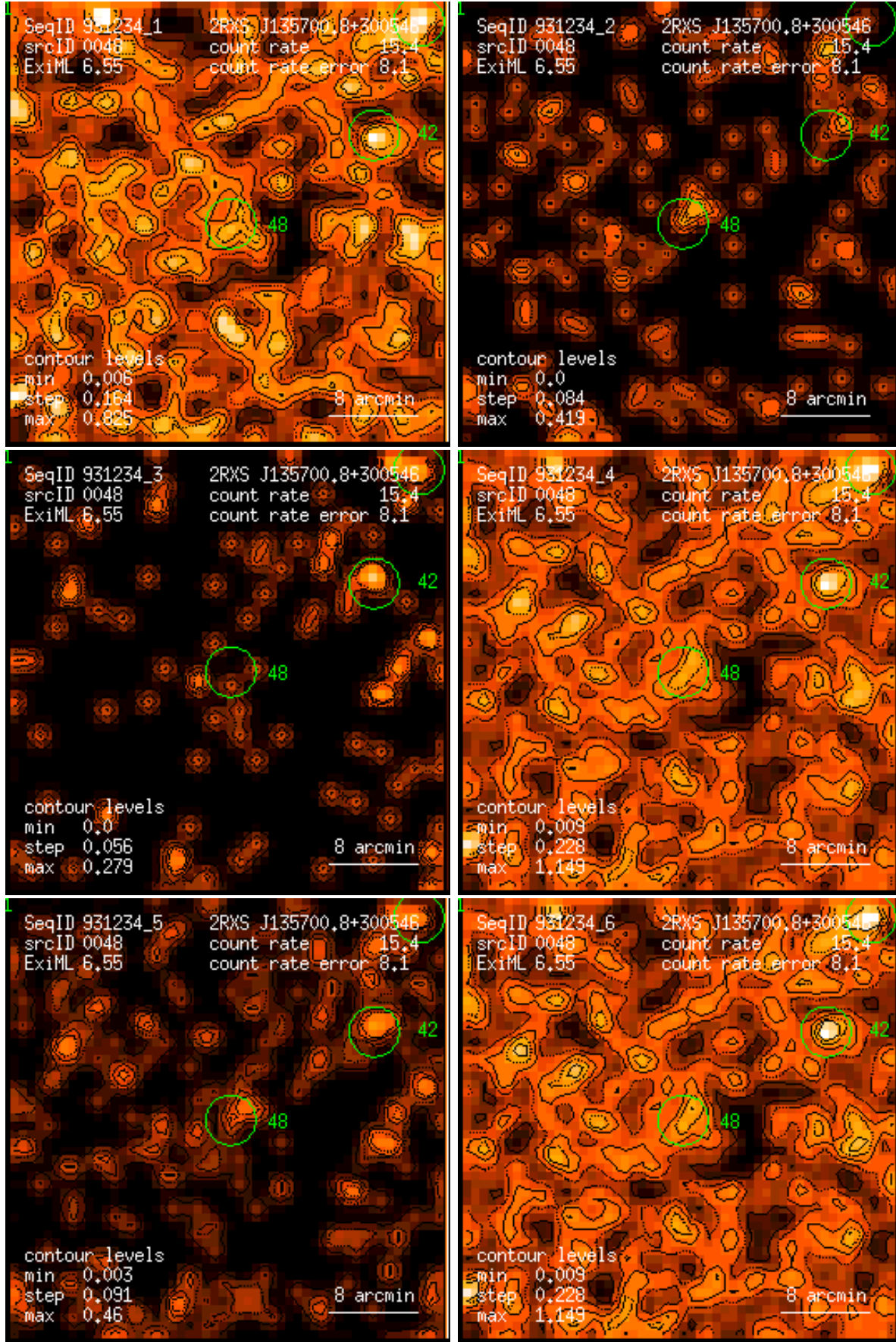
Figure 48: RASS 931234: detection 0048: band rate images, Gaussian filter: (1) PSPC channels 11 – 41, (2) 52 – 90, (3) 91 – 201, (4) 11 – 235, (5) 52 – 201, (6) 11 – 201. Broad band rates in counts/ks. Band rate contour levels in counts/ks/arcmin 2 .
