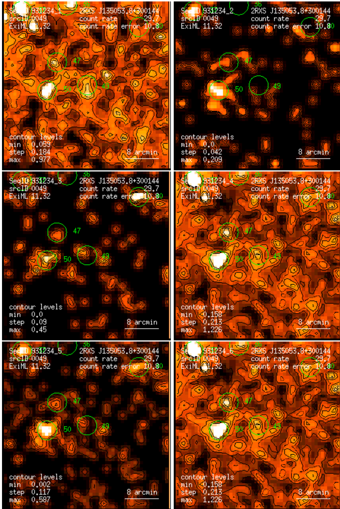
Figure 49: RASS 931234: detection 0049: band rate images, Gaussian filter: (1) PSPC channels 11 – 41, (2) 52 – 90, (3) 91 – 201, (4) 11 – 235, (5) 52 – 201, (6) 11 – 201. Broad band rates in counts/ks. Band rate contour levels in counts/ks/arcmin 2 .
