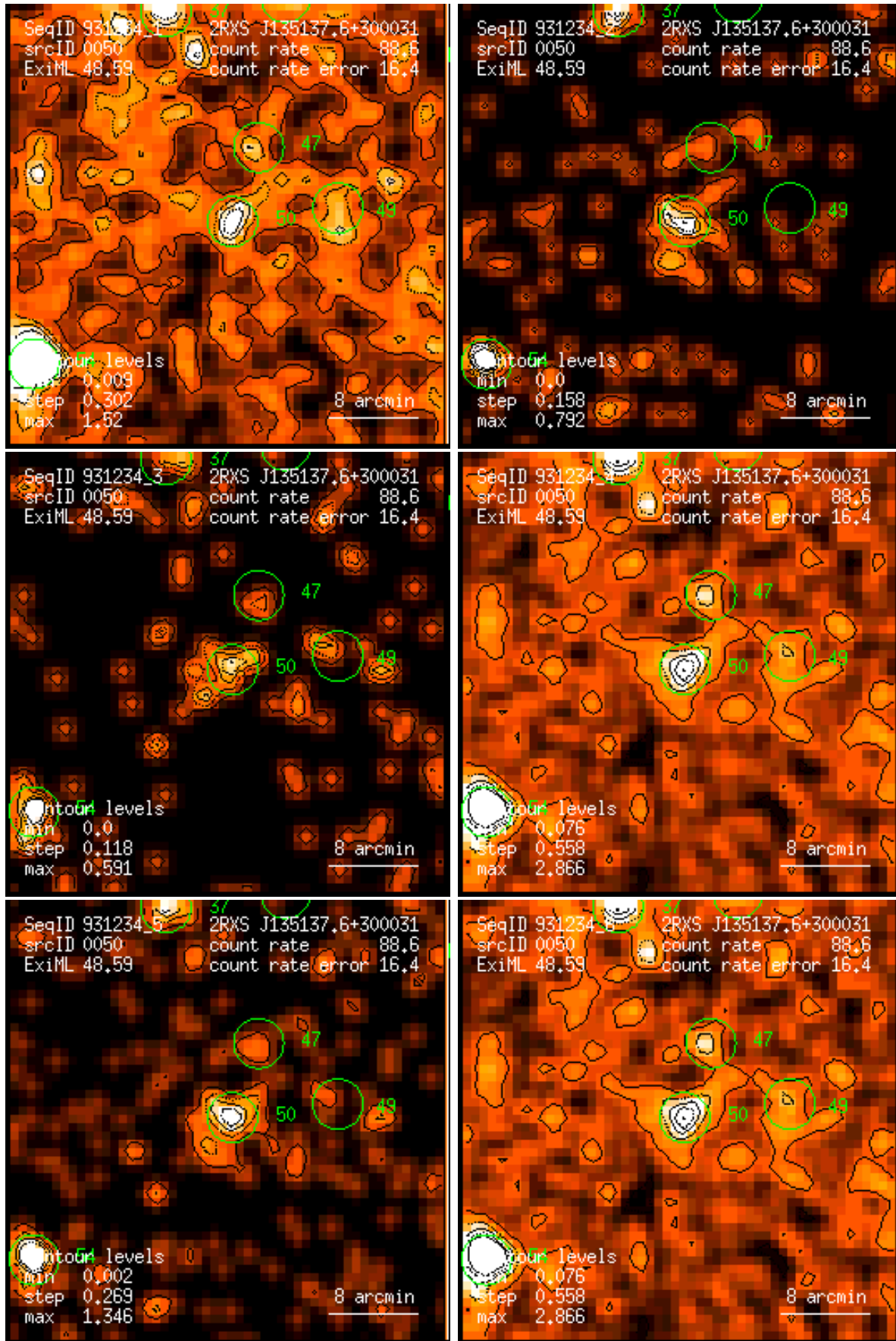
Figure 50: RASS 931234: detection 0050: band rate images, Gaussian filter: (1) PSPC channels 11 – 41, (2) 52 – 90, (3) 91 – 201, (4) 11 – 235, (5) 52 – 201, (6) 11 – 201. Broad band rates in counts/ks. Band rate contour levels in counts/ks/arcmin 2 .
