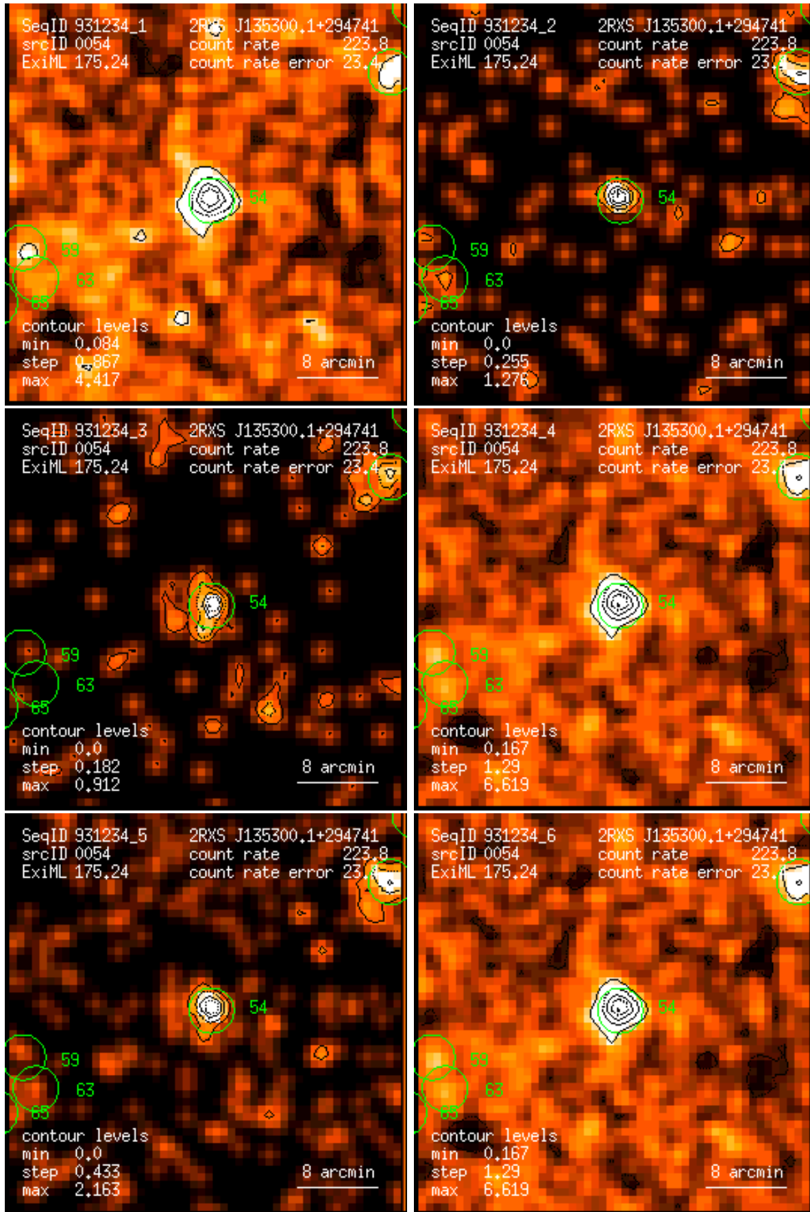
Figure 54: RASS 931234: detection 0054: band rate images, Gaussian filter: (1) PSPC channels 11 – 41, (2) 52 – 90, (3) 91 – 201, (4) 11 – 235, (5) 52 – 201, (6) 11 – 201. Broad band rates in counts/ks. Band rate contour levels in counts/ks/arcmin 2 .
