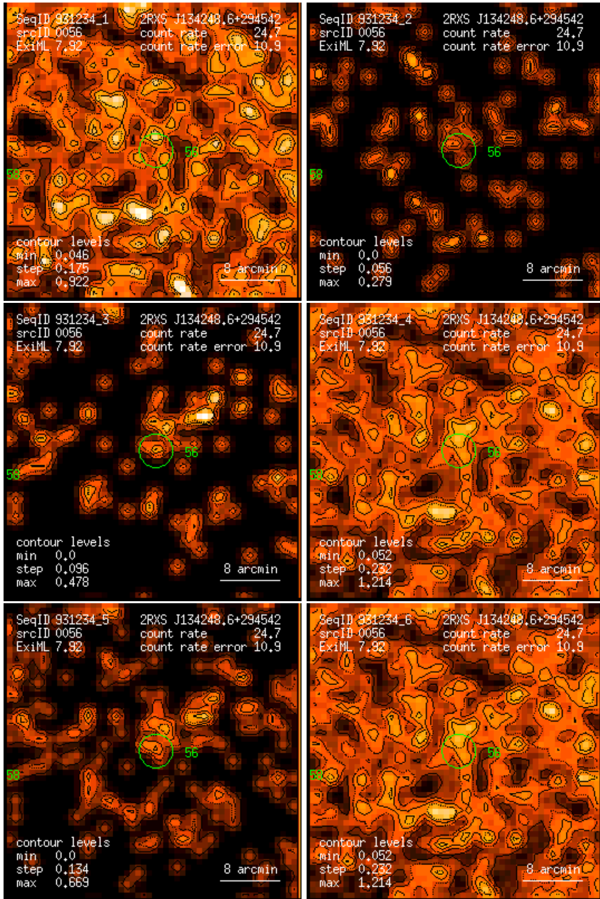
Figure 56: RASS 931234: detection 0056: band rate images, Gaussian filter: (1) PSPC channels 11 – 41, (2) 52 – 90, (3) 91 – 201, (4) 11 – 235, (5) 52 – 201, (6) 11 – 201. Broad band rates in counts/ks. Band rate contour levels in counts/ks/arcmin 2 .
