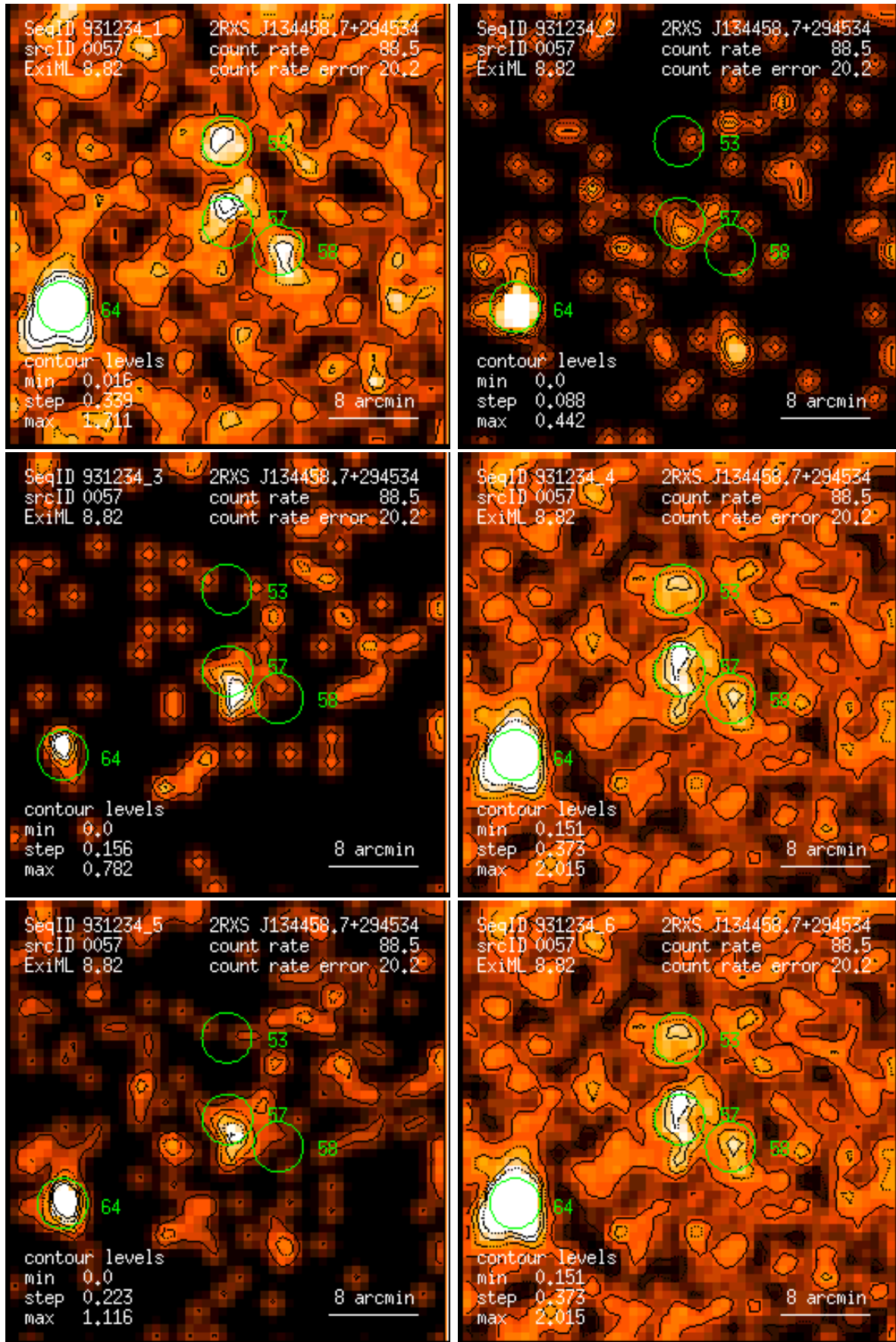
Figure 57: RASS 931234: detection 0057: band rate images, Gaussian filter: (1) PSPC channels 11 – 41, (2) 52 – 90, (3) 91 – 201, (4) 11 – 235, (5) 52 – 201, (6) 11 – 201. Broad band rates in counts/ks. Band rate contour levels in counts/ks/arcmin 2 .
