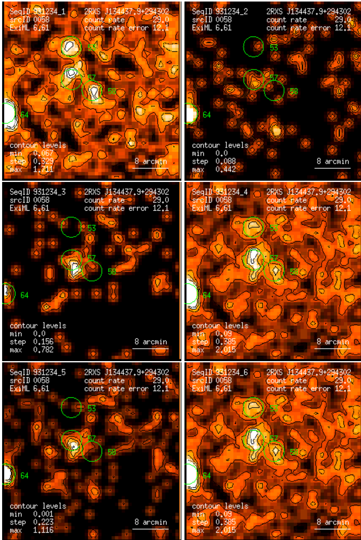
Figure 58: RASS 931234: detection 0058: band rate images, Gaussian filter: (1) PSPC channels 11 – 41, (2) 52 – 90, (3) 91 – 201, (4) 11 – 235, (5) 52 – 201, (6) 11 – 201. Broad band rates in counts/ks. Band rate contour levels in counts/ks/arcmin 2 .
