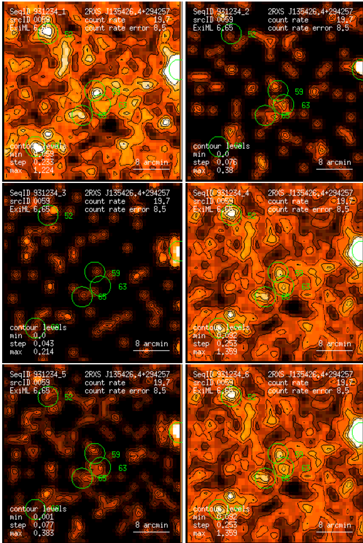
Figure 59: RASS 931234: detection 0059: band rate images, Gaussian filter: (1) PSPC channels 11 – 41, (2) 52 – 90, (3) 91 – 201, (4) 11 – 235, (5) 52 – 201, (6) 11 – 201. Broad band rates in counts/ks. Band rate contour levels in counts/ks/arcmin 2 .
