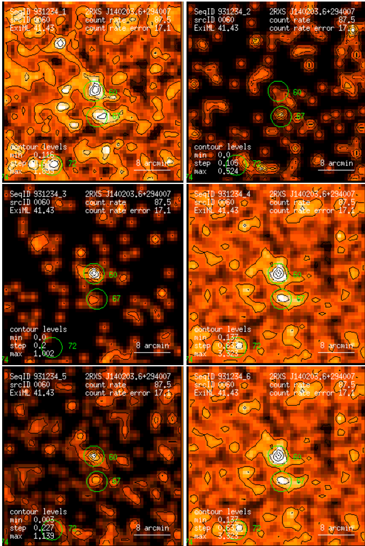
Figure 60: RASS 931234: detection 0060: band rate images, Gaussian filter: (1) PSPC channels 11 – 41, (2) 52 – 90, (3) 91 – 201, (4) 11 – 235, (5) 52 – 201, (6) 11 – 201. Broad band rates in counts/ks. Band rate contour levels in counts/ks/arcmin 2 .
