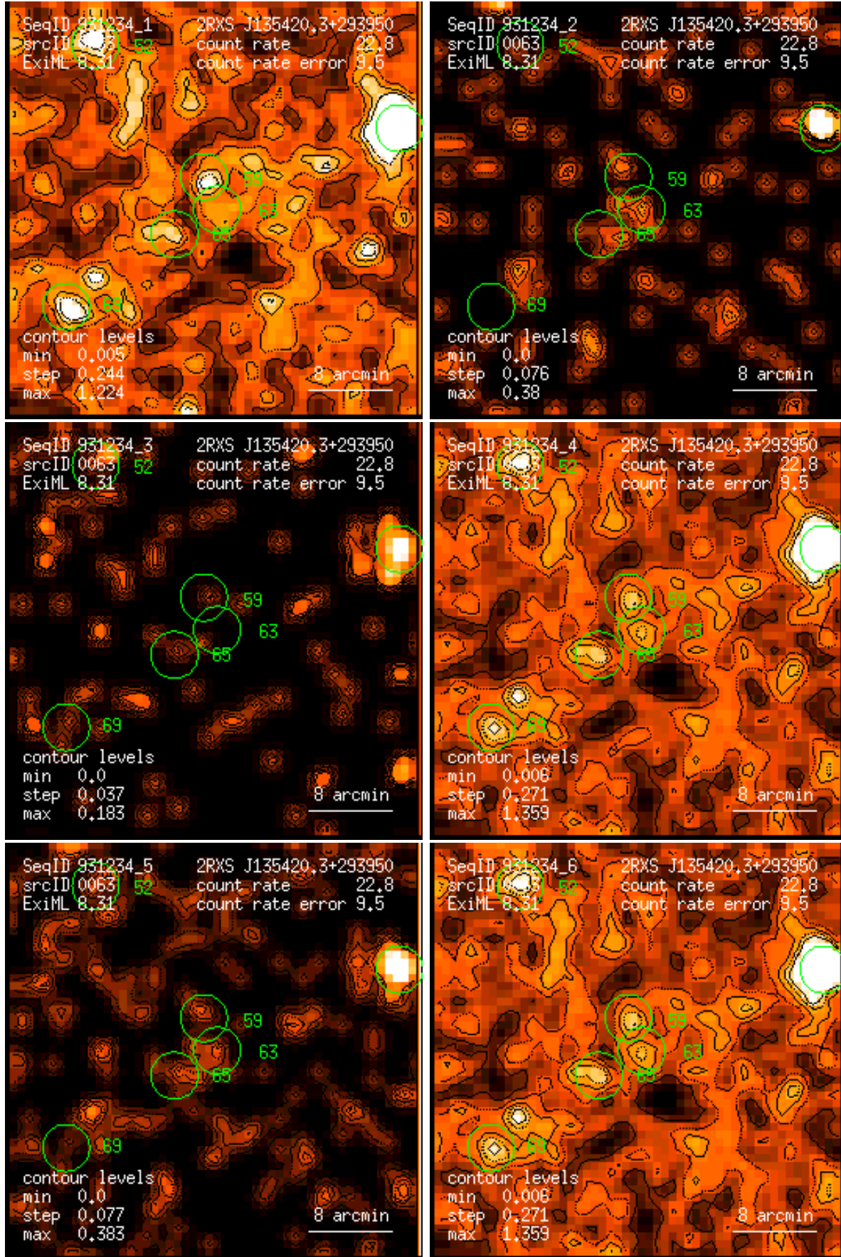
Figure 63: RASS 931234: detection 0063: band rate images, Gaussian filter: (1) PSPC channels 11 – 41, (2) 52 – 90, (3) 91 – 201, (4) 11 – 235, (5) 52 – 201, (6) 11 – 201. Broad band rates in counts/ks. Band rate contour levels in counts/ks/arcmin 2 .
