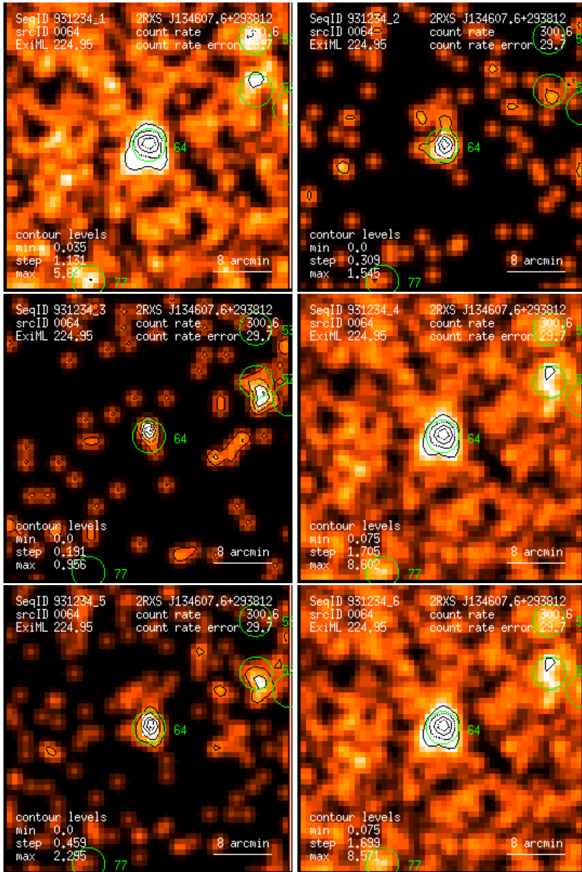
Figure 64: RASS 931234: detection 0064: band rate images, Gaussian filter: (1) PSPC channels 11 – 41, (2) 52 – 90, (3) 91 – 201, (4) 11 – 235, (5) 52 – 201, (6) 11 – 201. Broad band rates in counts/ks. Band rate contour levels in counts/ks/arcmin 2 .
