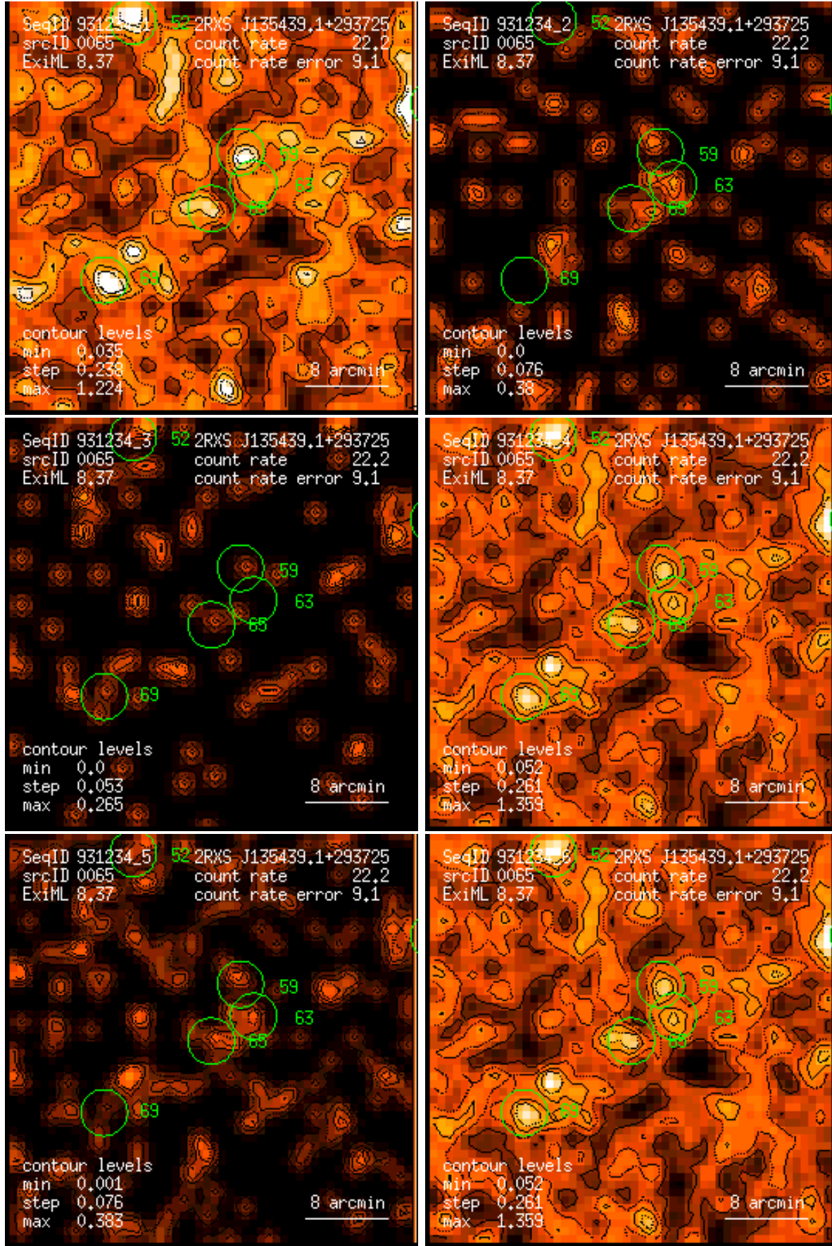
Figure 65: RASS 931234: detection 0065: band rate images, Gaussian filter: (1) PSPC channels 11 – 41, (2) 52 – 90, (3) 91 – 201, (4) 11 – 235, (5) 52 – 201, (6) 11 – 201. Broad band rates in counts/ks. Band rate contour levels in counts/ks/arcmin 2 .
