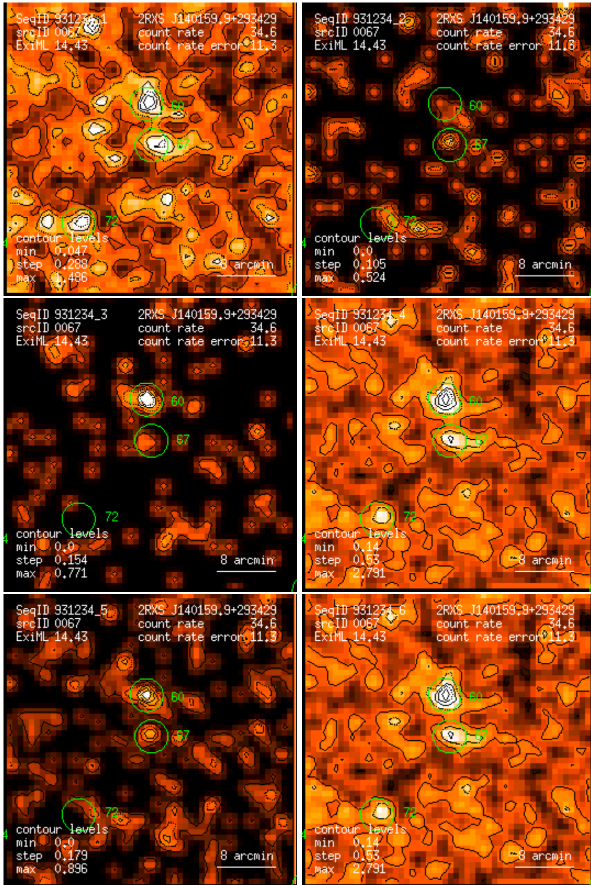
Figure 67: RASS 931234: detection 0067: band rate images, Gaussian filter: (1) PSPC channels 11 – 41, (2) 52 – 90, (3) 91 – 201, (4) 11 – 235, (5) 52 – 201, (6) 11 – 201. Broad band rates in counts/ks. Band rate contour levels in counts/ks/arcmin 2 .
