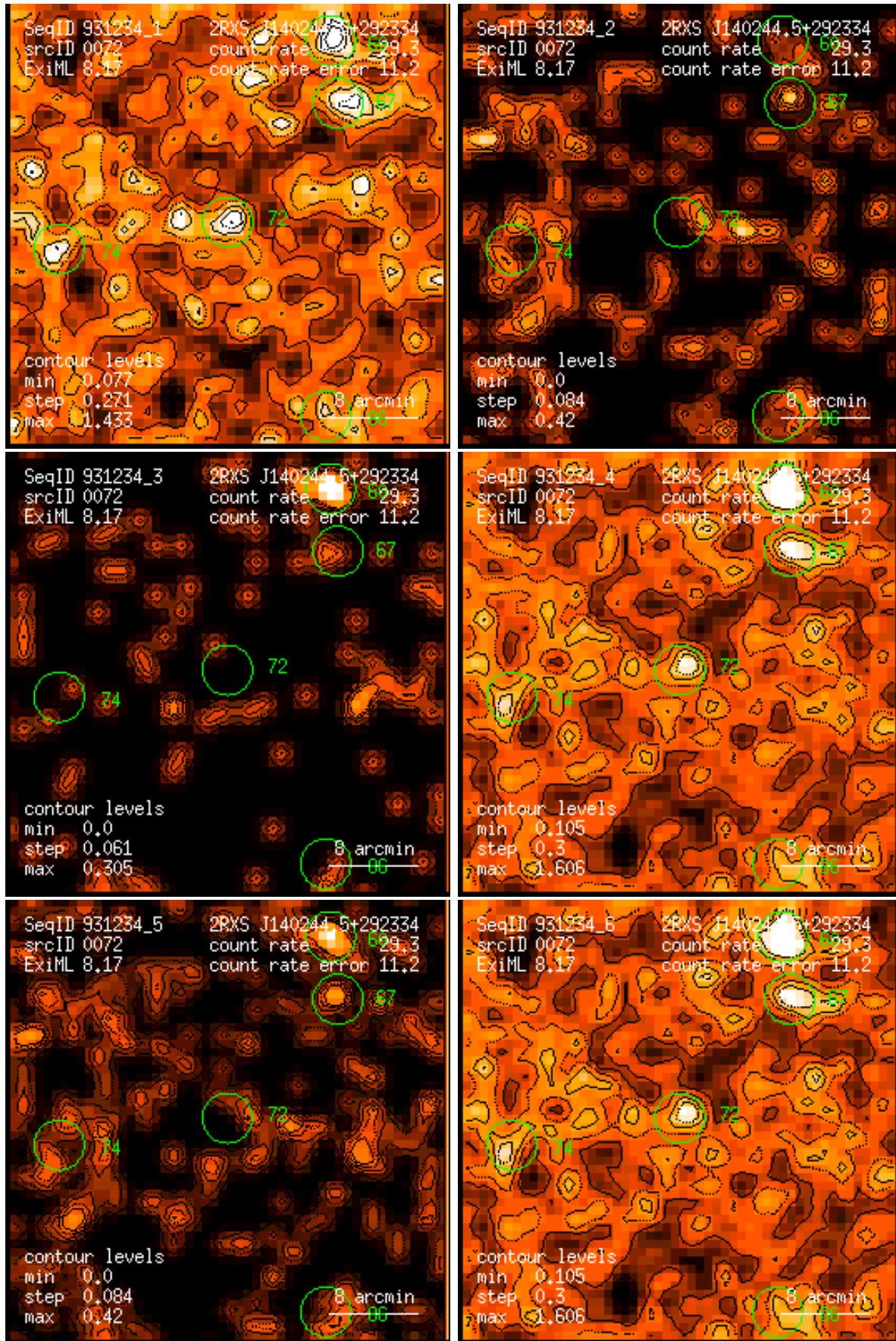
Figure 72: RASS 931234: detection 0072: band rate images, Gaussian filter: (1) PSPC channels 11 – 41, (2) 52 – 90, (3) 91 – 201, (4) 11 – 235, (5) 52 – 201, (6) 11 – 201. Broad band rates in counts/ks. Band rate contour levels in counts/ks/arcmin 2 .
