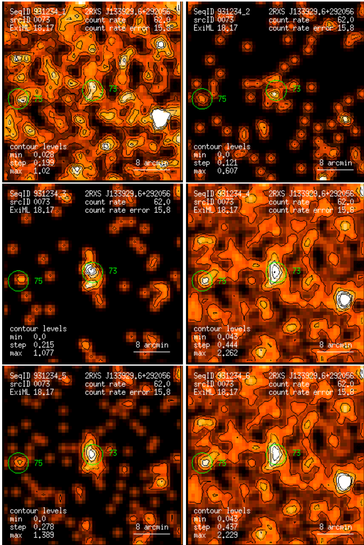
Figure 73: RASS 931234: detection 0073: band rate images, Gaussian filter: (1) PSPC channels 11 – 41, (2) 52 – 90, (3) 91 – 201, (4) 11 – 235, (5) 52 – 201, (6) 11 – 201. Broad band rates in counts/ks. Band rate contour levels in counts/ks/arcmin 2 .
