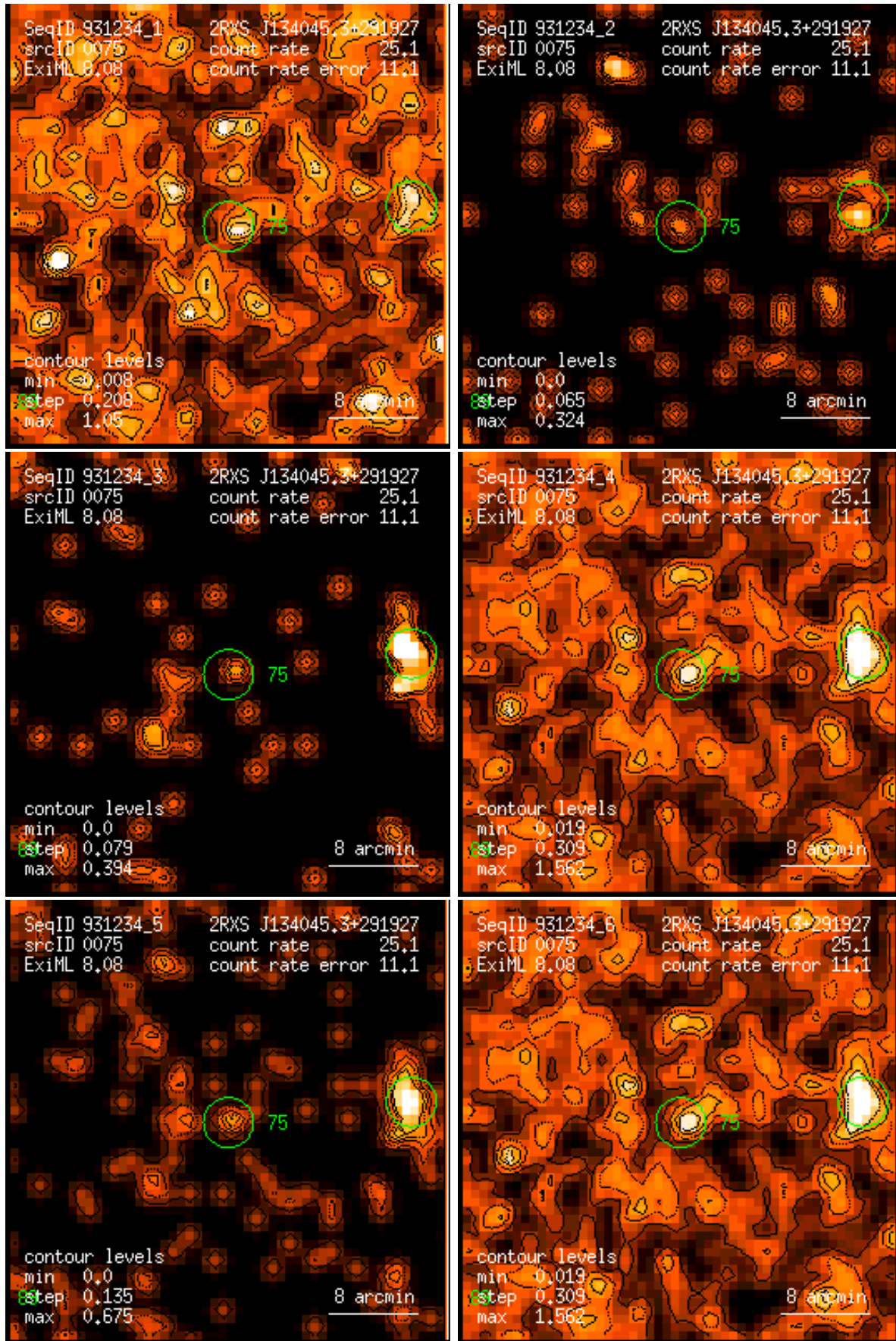
Figure 75: RASS 931234: detection 0075: band rate images, Gaussian filter: (1) PSPC channels 11 – 41, (2) 52 – 90, (3) 91 – 201, (4) 11 – 235, (5) 52 – 201, (6) 11 – 201. Broad band rates in counts/ks. Band rate contour levels in counts/ks/arcmin 2 .
