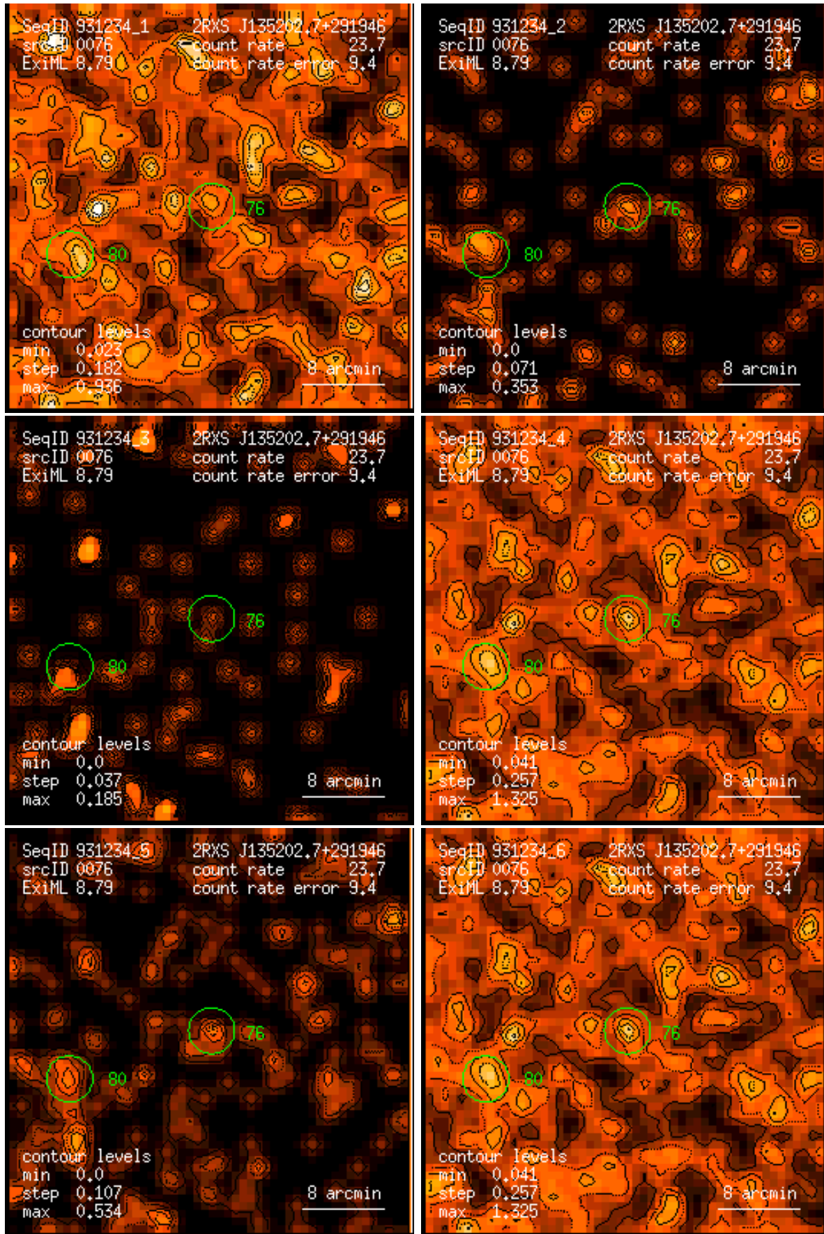
Figure 76: RASS 931234: detection 0076: band rate images, Gaussian filter: (1) PSPC channels 11 – 41, (2) 52 – 90, (3) 91 – 201, (4) 11 – 235, (5) 52 – 201, (6) 11 – 201. Broad band rates in counts/ks. Band rate contour levels in counts/ks/arcmin 2 .
