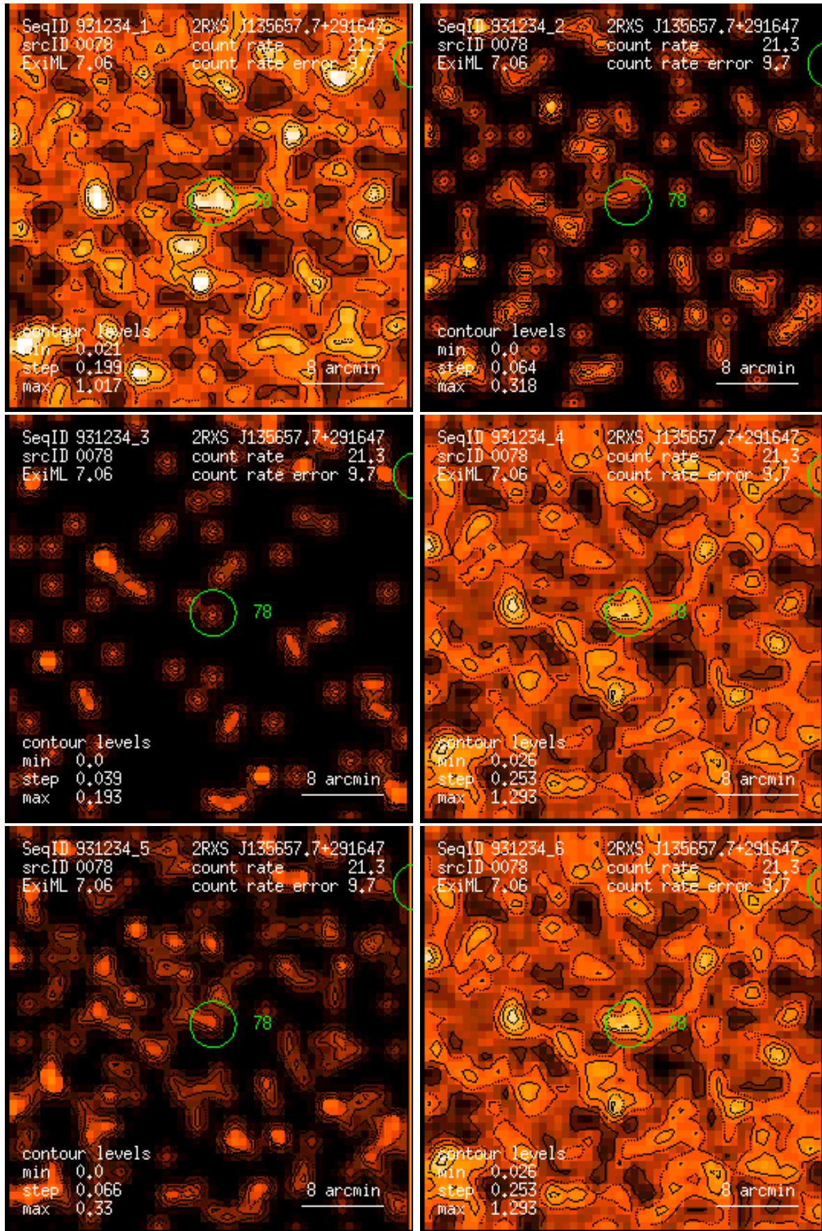
Figure 78: RASS 931234: detection 0078: band rate images, Gaussian filter: (1) PSPC channels 11 – 41, (2) 52 – 90, (3) 91 – 201, (4) 11 – 235, (5) 52 – 201, (6) 11 – 201. Broad band rates in counts/ks. Band rate contour levels in counts/ks/arcmin 2 .
