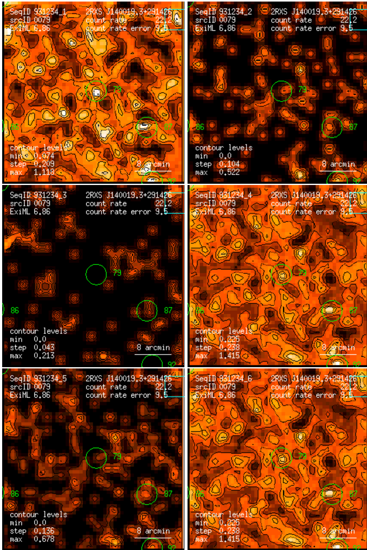
Figure 79: RASS 931234: detection 0079: band rate images, Gaussian filter: (1) PSPC channels 11 – 41, (2) 52 – 90, (3) 91 – 201, (4) 11 – 235, (5) 52 – 201, (6) 11 – 201. Broad band rates in counts/ks. Band rate contour levels in counts/ks/arcmin 2 .
