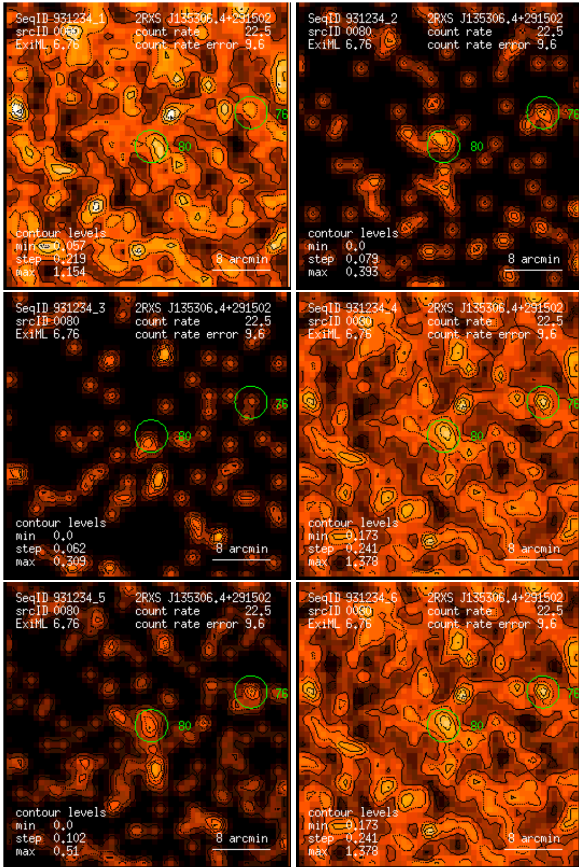
Figure 80: RASS 931234: detection 0080: band rate images, Gaussian filter: (1) PSPC channels 11 – 41, (2) 52 – 90, (3) 91 – 201, (4) 11 – 235, (5) 52 – 201, (6) 11 – 201. Broad band rates in counts/ks. Band rate contour levels in counts/ks/arcmin 2 .
