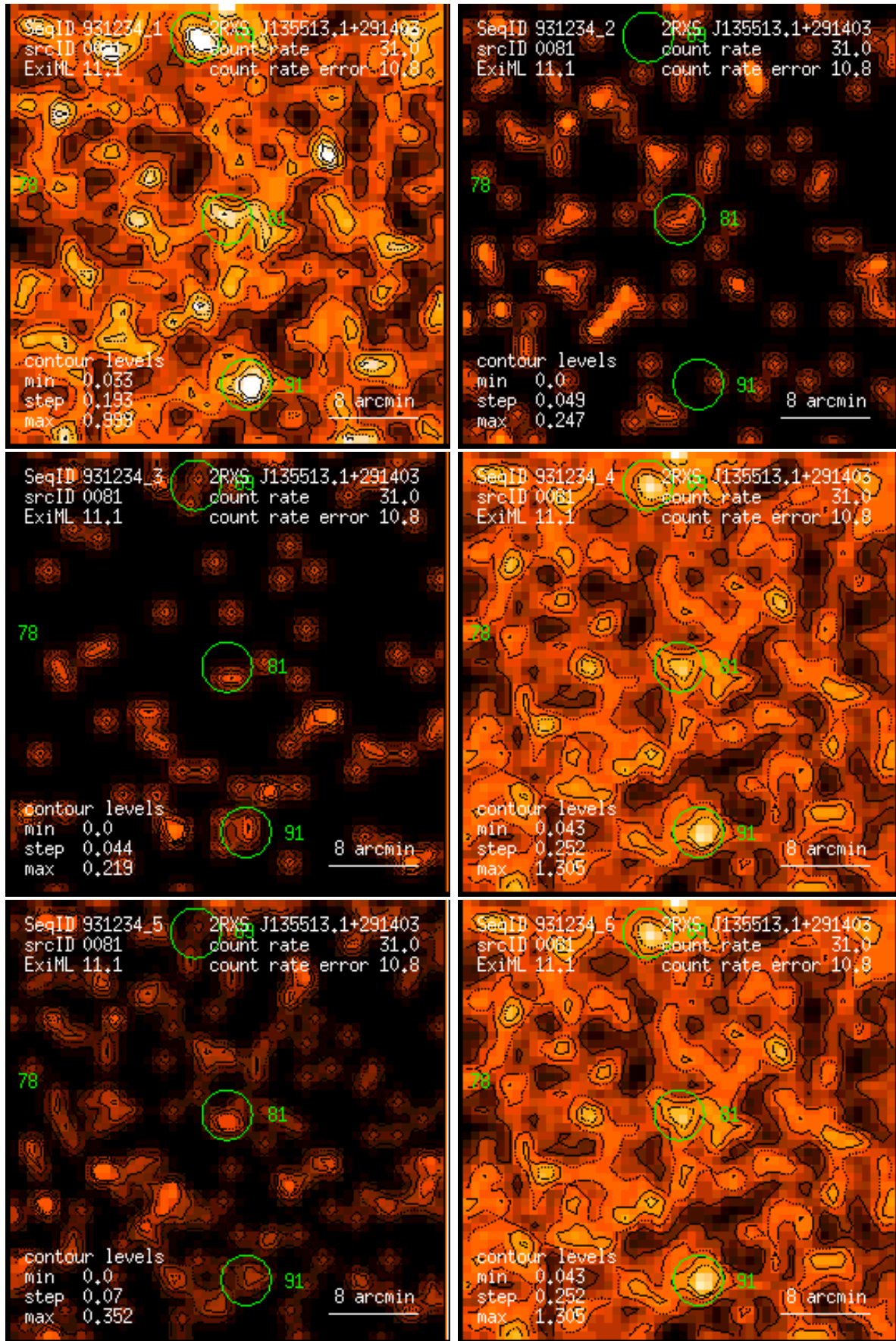
Figure 81: RASS 931234: detection 0081: band rate images, Gaussian filter: (1) PSPC channels 11 – 41, (2) 52 – 90, (3) 91 – 201, (4) 11 – 235, (5) 52 – 201, (6) 11 – 201. Broad band rates in counts/ks. Band rate contour levels in counts/ks/arcmin 2 .
