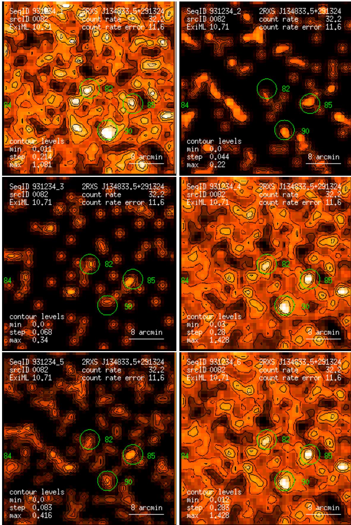
Figure 82: RASS 931234: detection 0082: band rate images, Gaussian filter: (1) PSPC channels 11 – 41, (2) 52 – 90, (3) 91 – 201, (4) 11 – 235, (5) 52 – 201, (6) 11 – 201. Broad band rates in counts/ks. Band rate contour levels in counts/ks/arcmin 2 .
