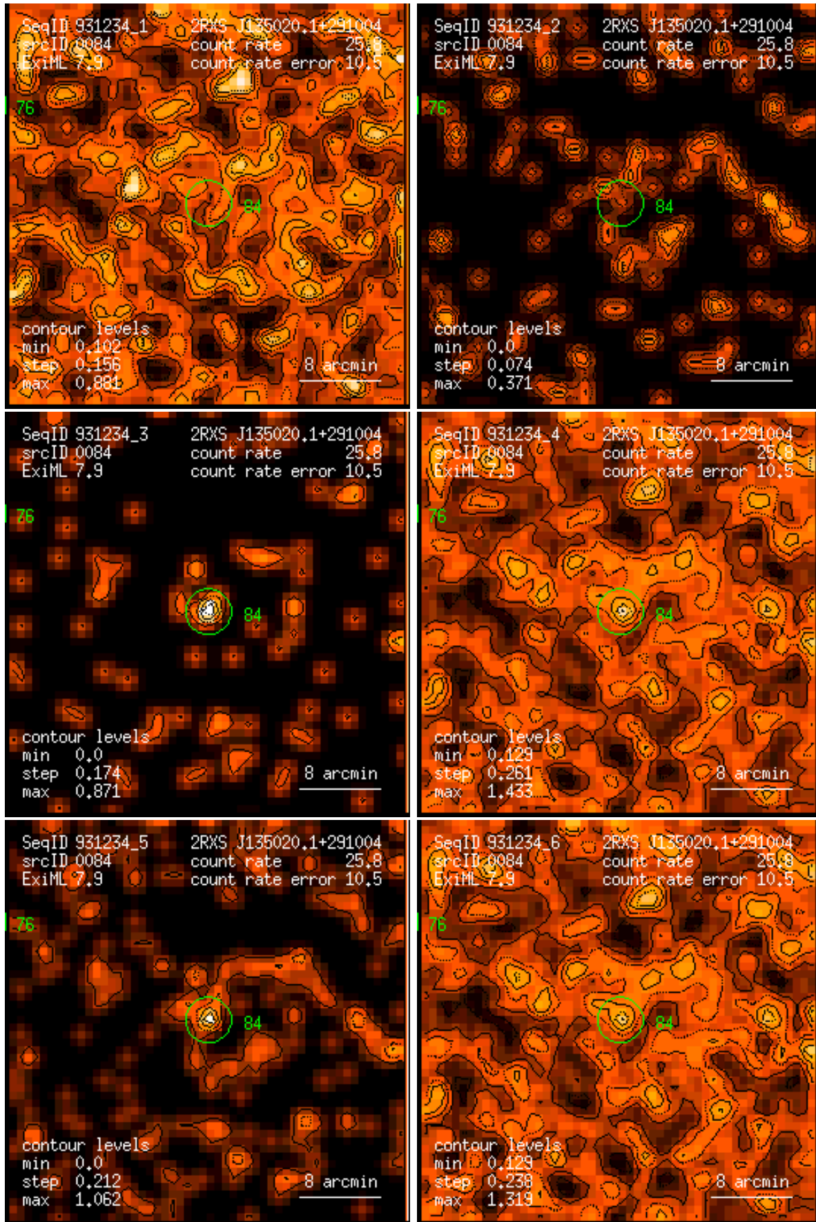
Figure 84: RASS 931234: detection 0084: band rate images, Gaussian filter: (1) PSPC channels 11 – 41, (2) 52 – 90, (3) 91 – 201, (4) 11 – 235, (5) 52 – 201, (6) 11 – 201. Broad band rates in counts/ks. Band rate contour levels in counts/ks/arcmin 2 .
