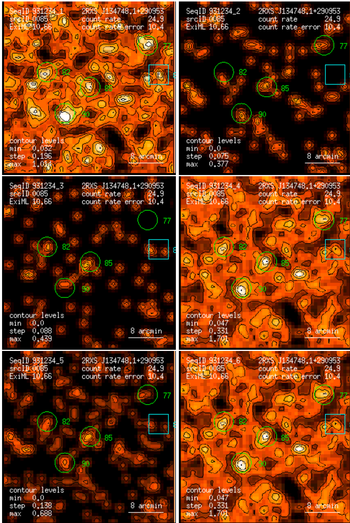
Figure 85: RASS 931234: detection 0085: band rate images, Gaussian filter: (1) PSPC channels 11 – 41, (2) 52 – 90, (3) 91 – 201, (4) 11 – 235, (5) 52 – 201, (6) 11 – 201. Broad band rates in counts/ks. Band rate contour levels in counts/ks/arcmin 2 .
