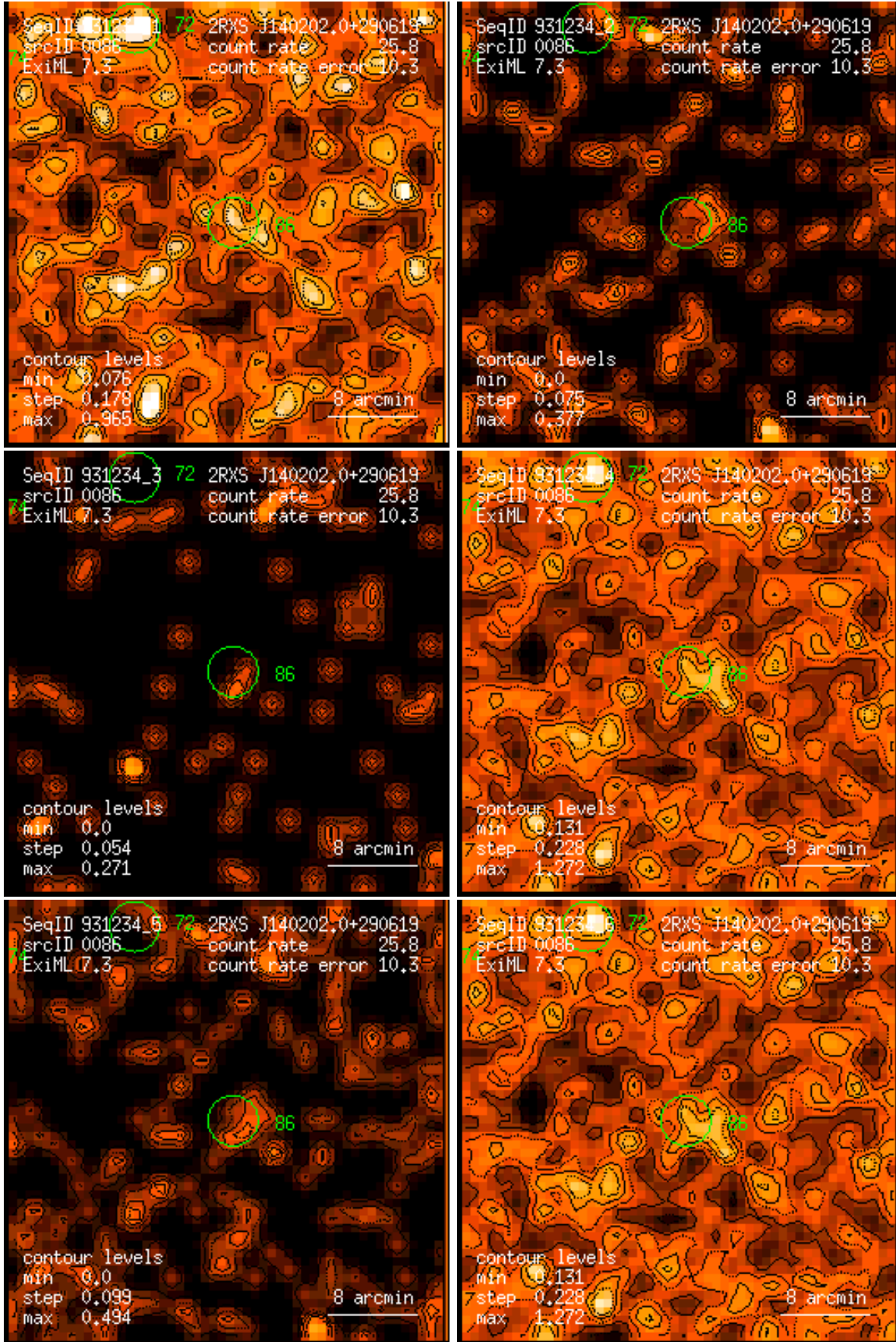
Figure 86: RASS 931234: detection 0086: band rate images, Gaussian filter: (1) PSPC channels 11 – 41, (2) 52 – 90, (3) 91 – 201, (4) 11 – 235, (5) 52 – 201, (6) 11 – 201. Broad band rates in counts/ks. Band rate contour levels in counts/ks/arcmin 2 .
