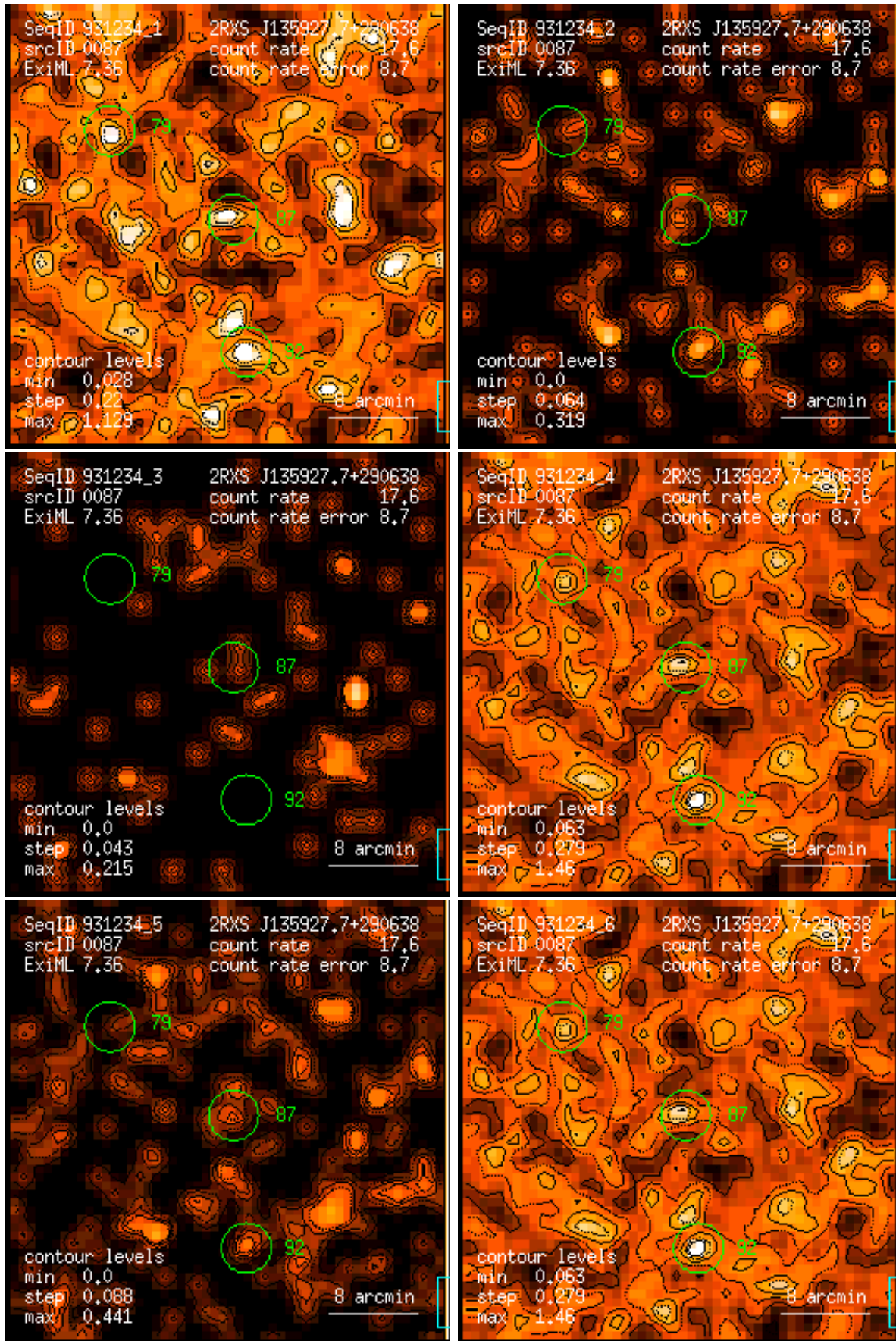
Figure 87: RASS 931234: detection 0087: band rate images, Gaussian filter: (1) PSPC channels 11 – 41, (2) 52 – 90, (3) 91 – 201, (4) 11 – 235, (5) 52 – 201, (6) 11 – 201. Broad band rates in counts/ks. Band rate contour levels in counts/ks/arcmin 2 .
