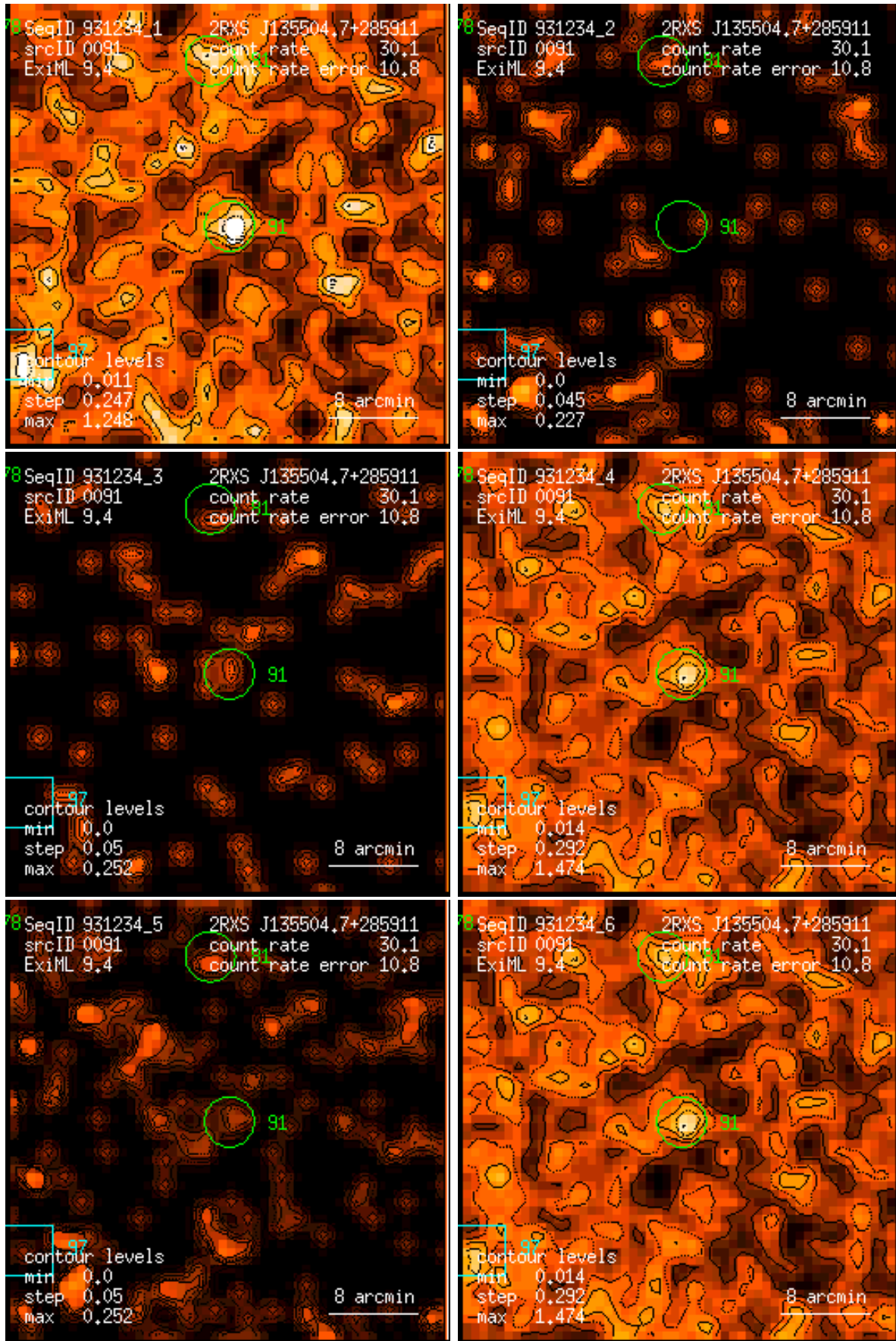
Figure 91: RASS 931234: detection 0091: band rate images, Gaussian filter: (1) PSPC channels 11 – 41, (2) 52 – 90, (3) 91 – 201, (4) 11 – 235, (5) 52 – 201, (6) 11 – 201. Broad band rates in counts/ks. Band rate contour levels in counts/ks/arcmin 2 .
