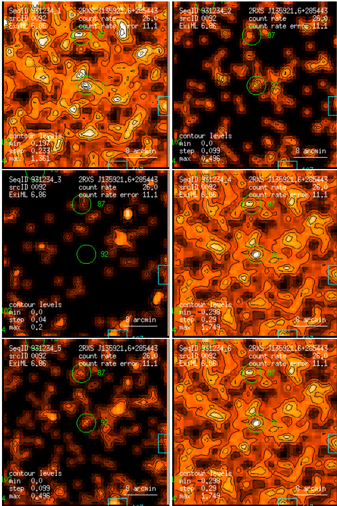
Figure 92: RASS 931234: detection 0092: band rate images, Gaussian filter: (1) PSPC channels 11 – 41, (2) 52 – 90, (3) 91 – 201, (4) 11 – 235, (5) 52 – 201, (6) 11 – 201. Broad band rates in counts/ks. Band rate contour levels in counts/ks/arcmin 2 .
