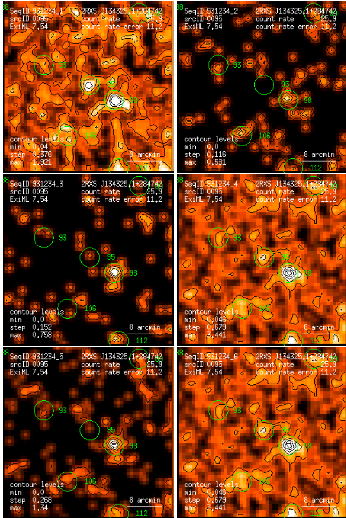
Figure 95: RASS 931234: detection 0095: band rate images, Gaussian filter: (1) PSPC channels 11 – 41, (2) 52 – 90, (3) 91 – 201, (4) 11 – 235, (5) 52 – 201, (6) 11 – 201. Broad band rates in counts/ks. Band rate contour levels in counts/ks/arcmin 2 .
