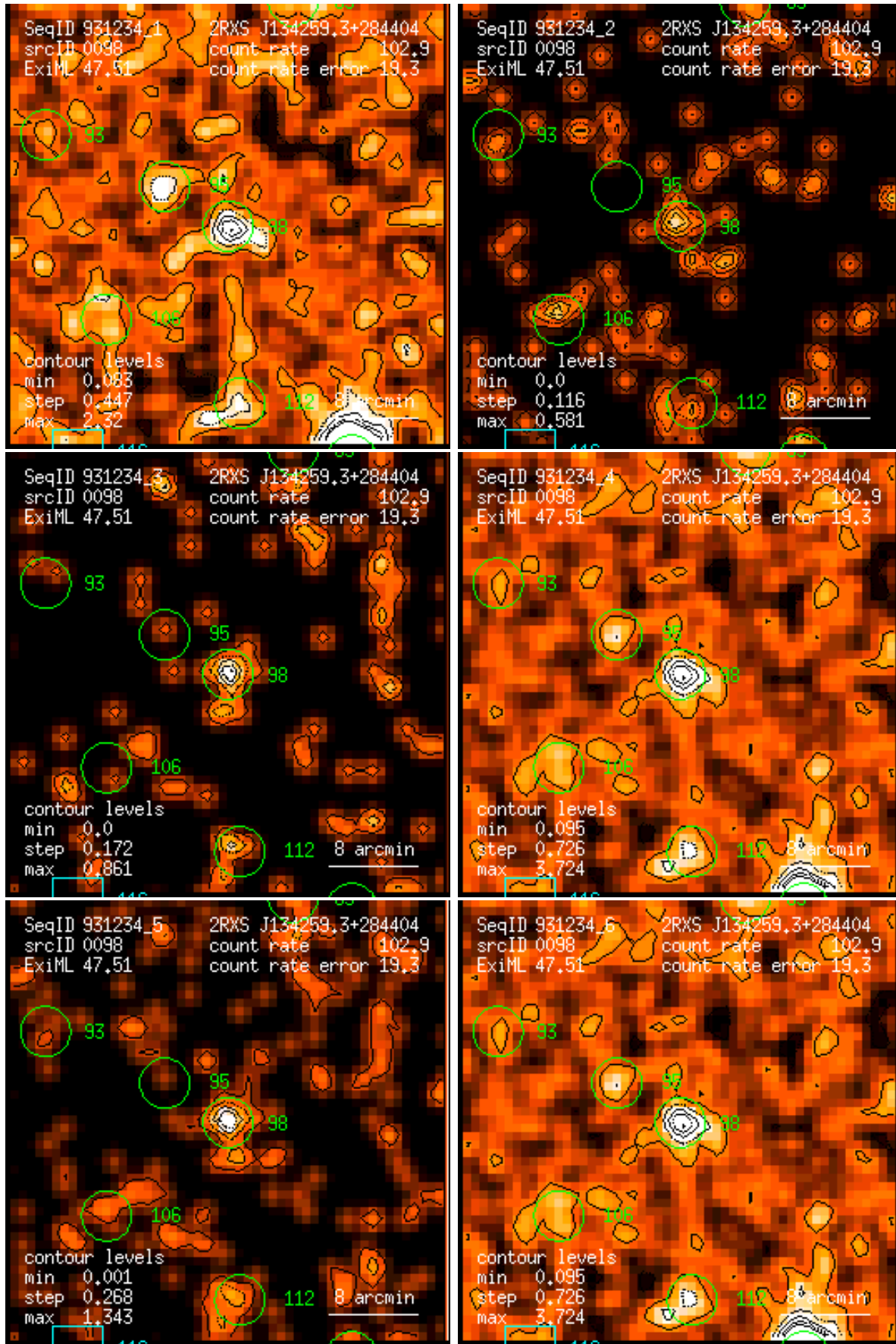
Figure 98: RASS 931234: detection 0098: band rate images, Gaussian filter: (1) PSPC channels 11 – 41, (2) 52 – 90, (3) 91 – 201, (4) 11 – 235, (5) 52 – 201, (6) 11 – 201. Broad band rates in counts/ks. Band rate contour levels in counts/ks/arcmin 2 .
