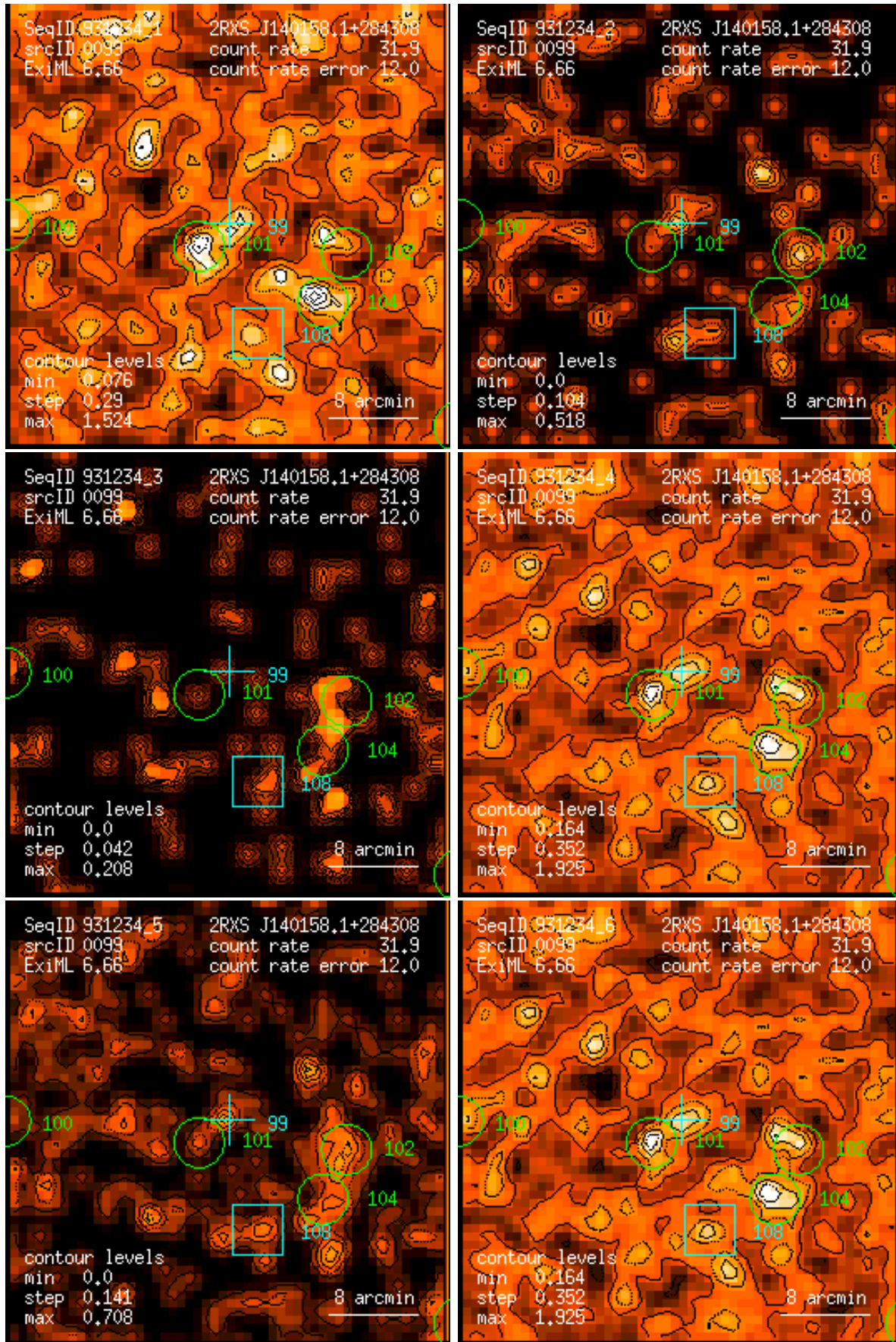
Figure 99: RASS 931234: detection 0099: band rate images, Gaussian filter: (1) PSPC channels 11 – 41, (2) 52 – 90, (3) 91 – 201, (4) 11 – 235, (5) 52 – 201, (6) 11 – 201. Broad band rates in counts/ks. Band rate contour levels in counts/ks/arcmin 2 .
