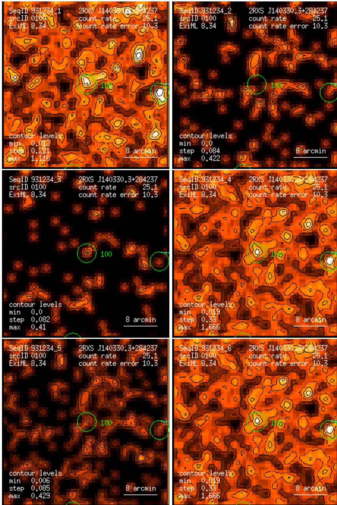
Figure 100: RASS 931234: detection 0100: band rate images, Gaussian filter: (1) PSPC channels 11 – 41, (2) 52 – 90, (3) 91 – 201, (4) 11 – 235, (5) 52 – 201, (6) 11 – 201. Broad band rates in counts/ks. Band rate contour levels in counts/ks/arcmin 2 .
