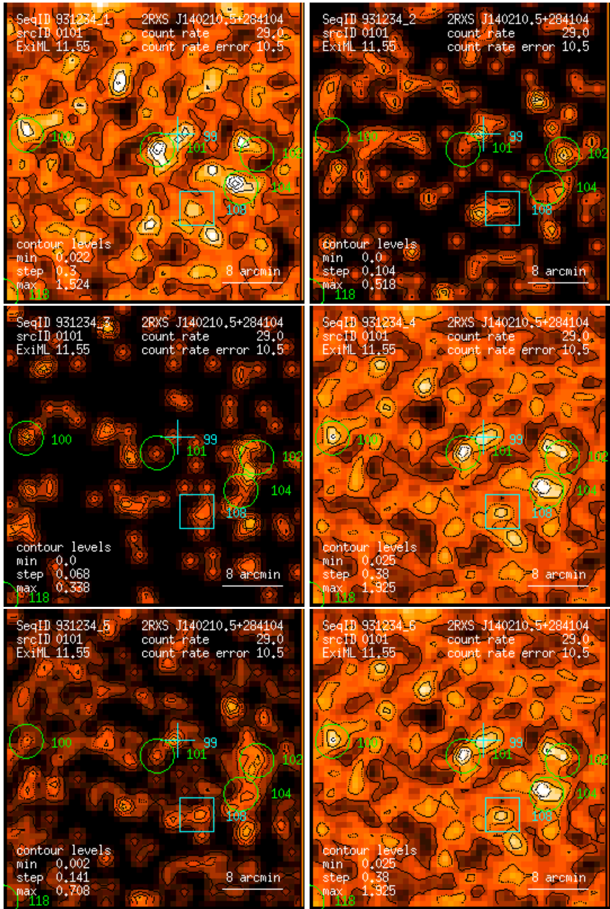
Figure 101: RASS 931234: detection 0101: band rate images, Gaussian filter: (1) PSPC channels 11 – 41, (2) 52 – 90, (3) 91 – 201, (4) 11 – 235, (5) 52 – 201, (6) 11 – 201. Broad band rates in counts/ks. Band rate contour levels in counts/ks/arcmin 2 .
